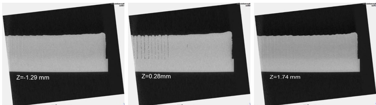
Figure 5: CT-Scans at three locations through the deposit. The center of the deposit was at approximately Z=0 mm.
