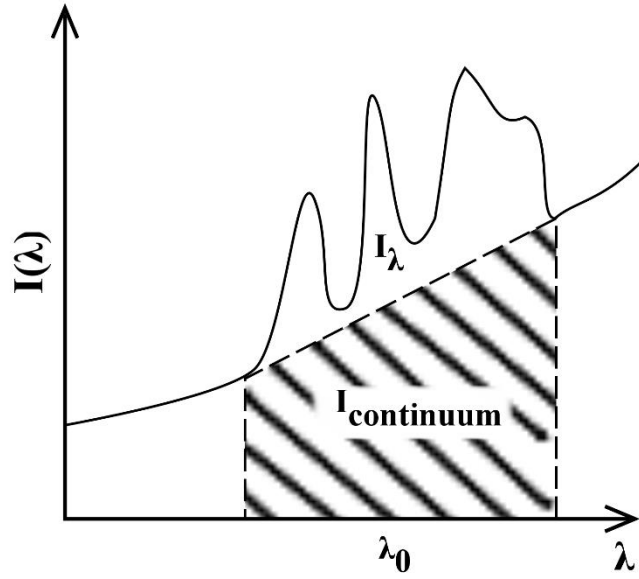
Figure 7: Definition of I_{\lambda} and I_{continuum} .
