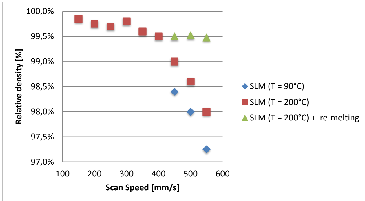
Figure 8: Influence of scan speed, pre-heating temperature and re-melting on part density
