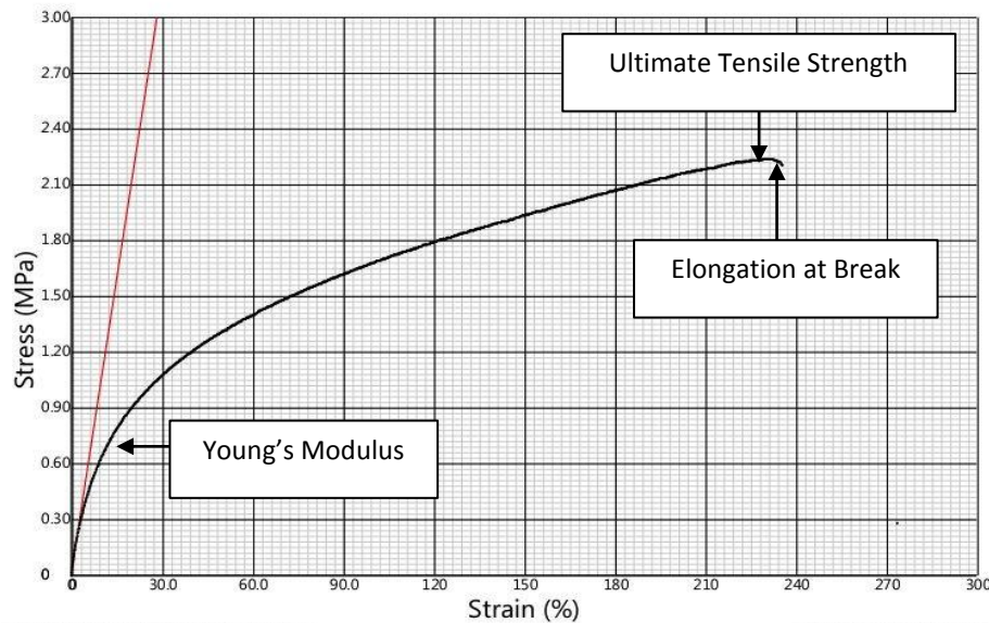
Figure 3 – EaB, YM and UTS determined from ASTM D638 Tensile Test
