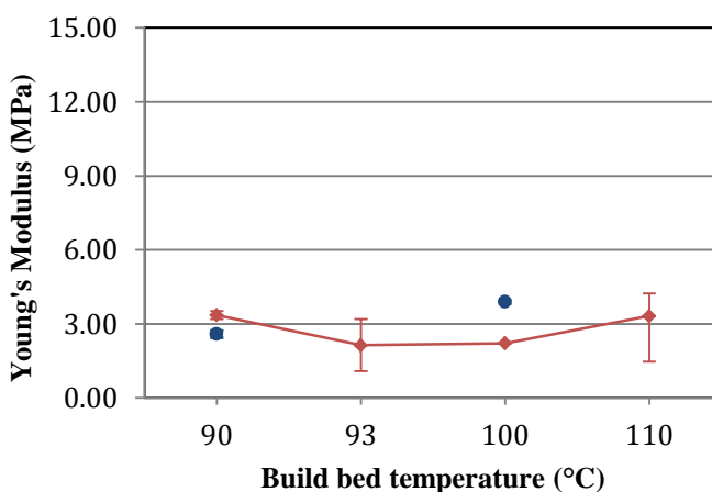
Figure 9 – Variation of YM with bed temperature
