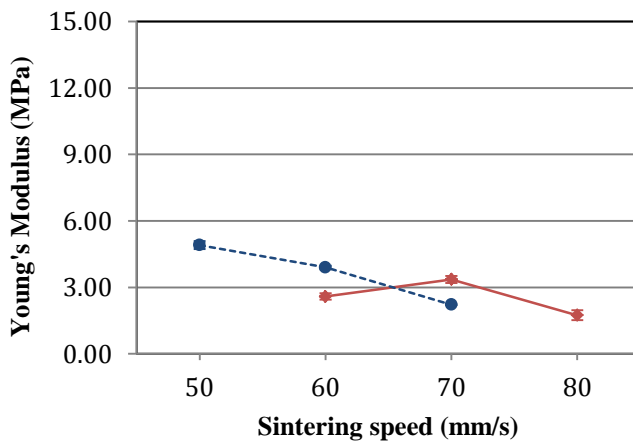
Figure 6 – Variation of YM with sintering speed
