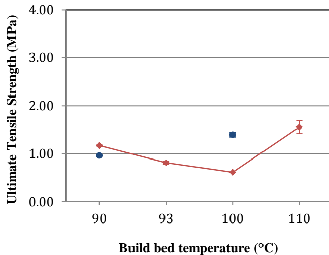
Figure 8 – Variation of UTS with bed temperature
