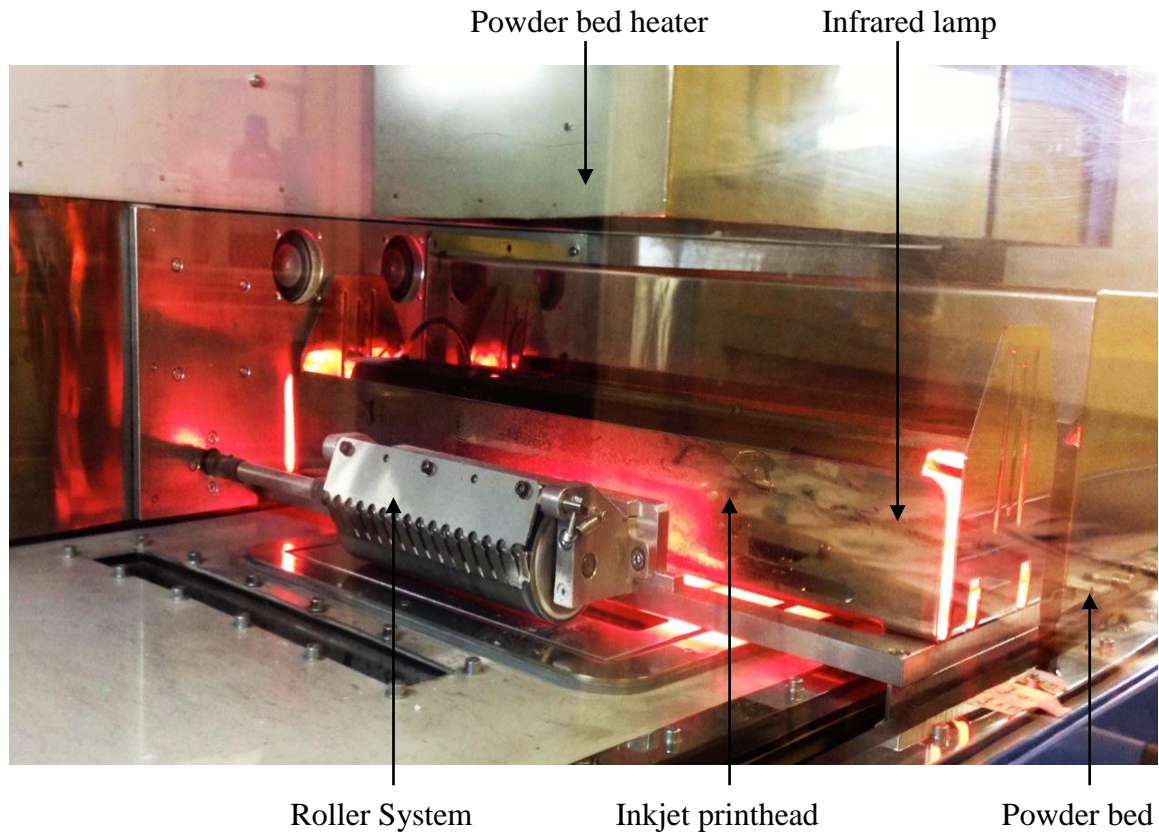
Figure 1 – High Speed Sintering machine and key parts
