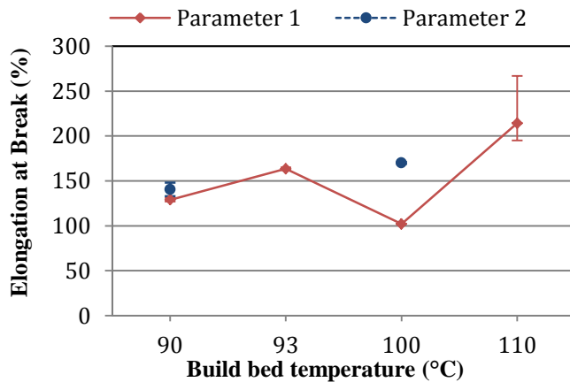
Figure 7 – Variation of EaB with bed temperature
