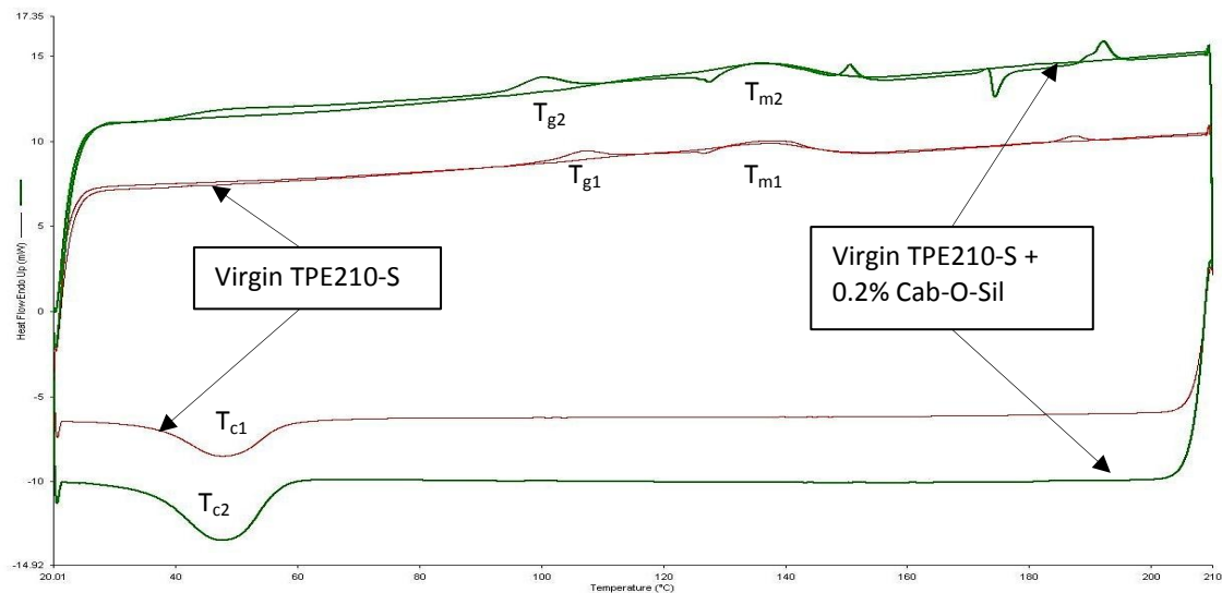
Figure 13 – DSC scan of TPE210-S mixed with 0.2% Cab-O-Sil and virgin TPE210-S
