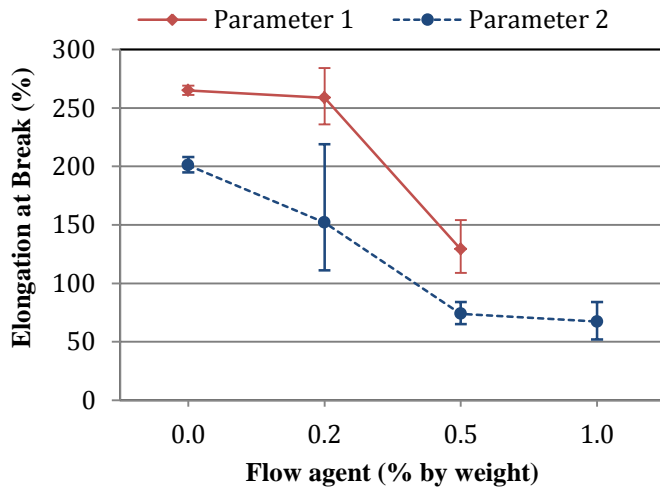
Figure 10 – Variation of EaB with flow agent level
