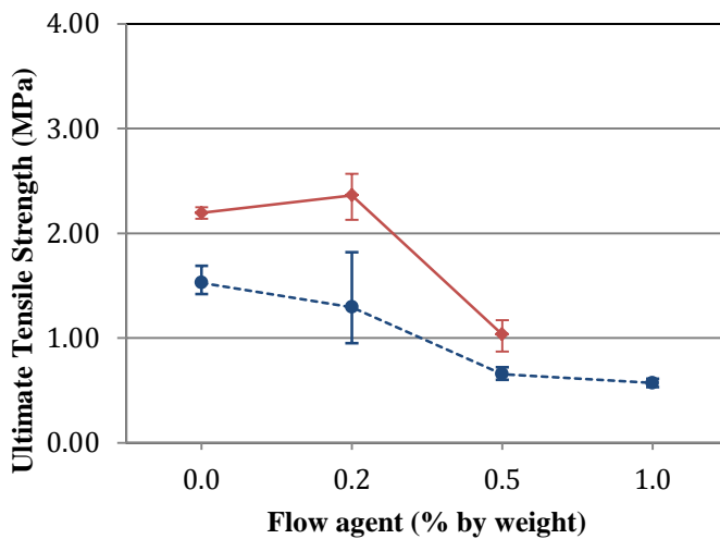
Figure 11 – Variation of UTS with flow agent level
