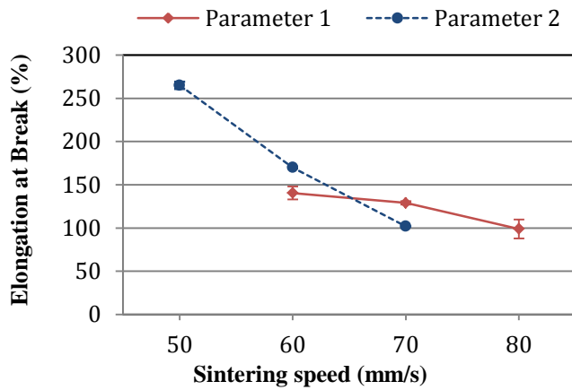
Figure 4 – Variation of EaB with sintering speed
