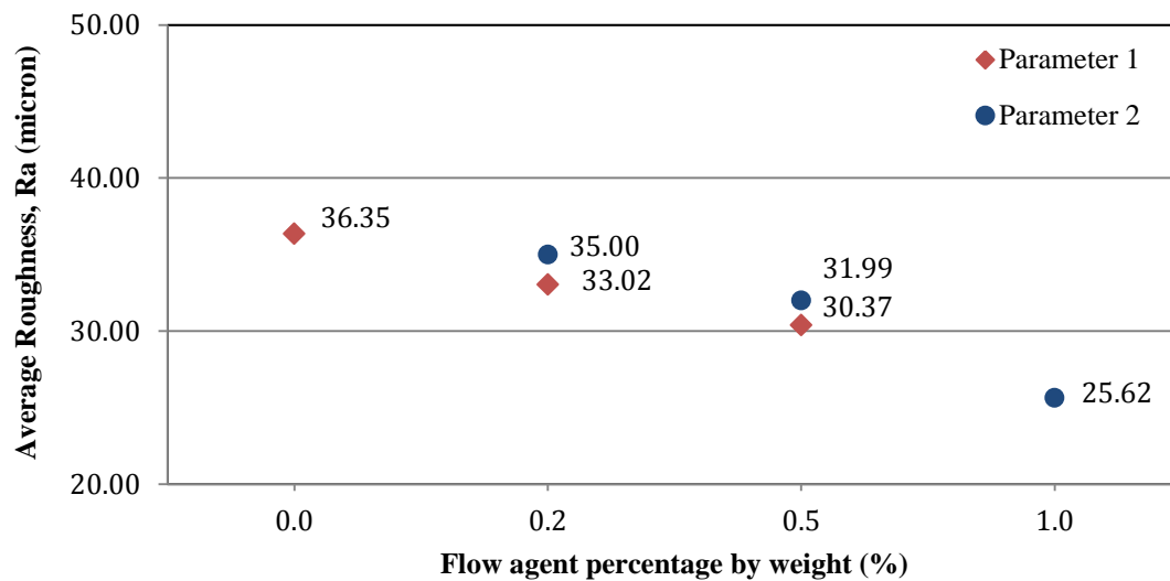
Figure 14 – Average roughness values against flow agent addition
