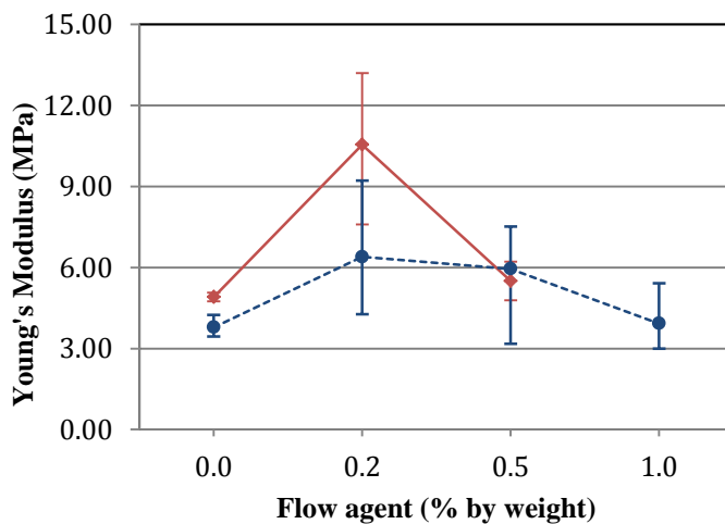
Figure 12 – Variation of YM with flow agent level
