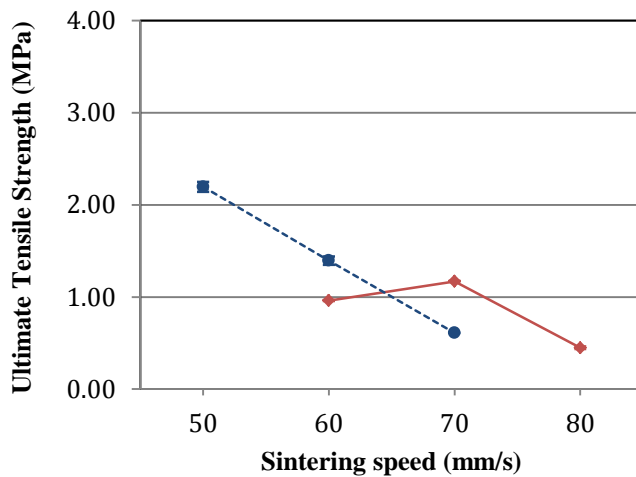
Figure 5 – Variation of UTS with sintering speed
