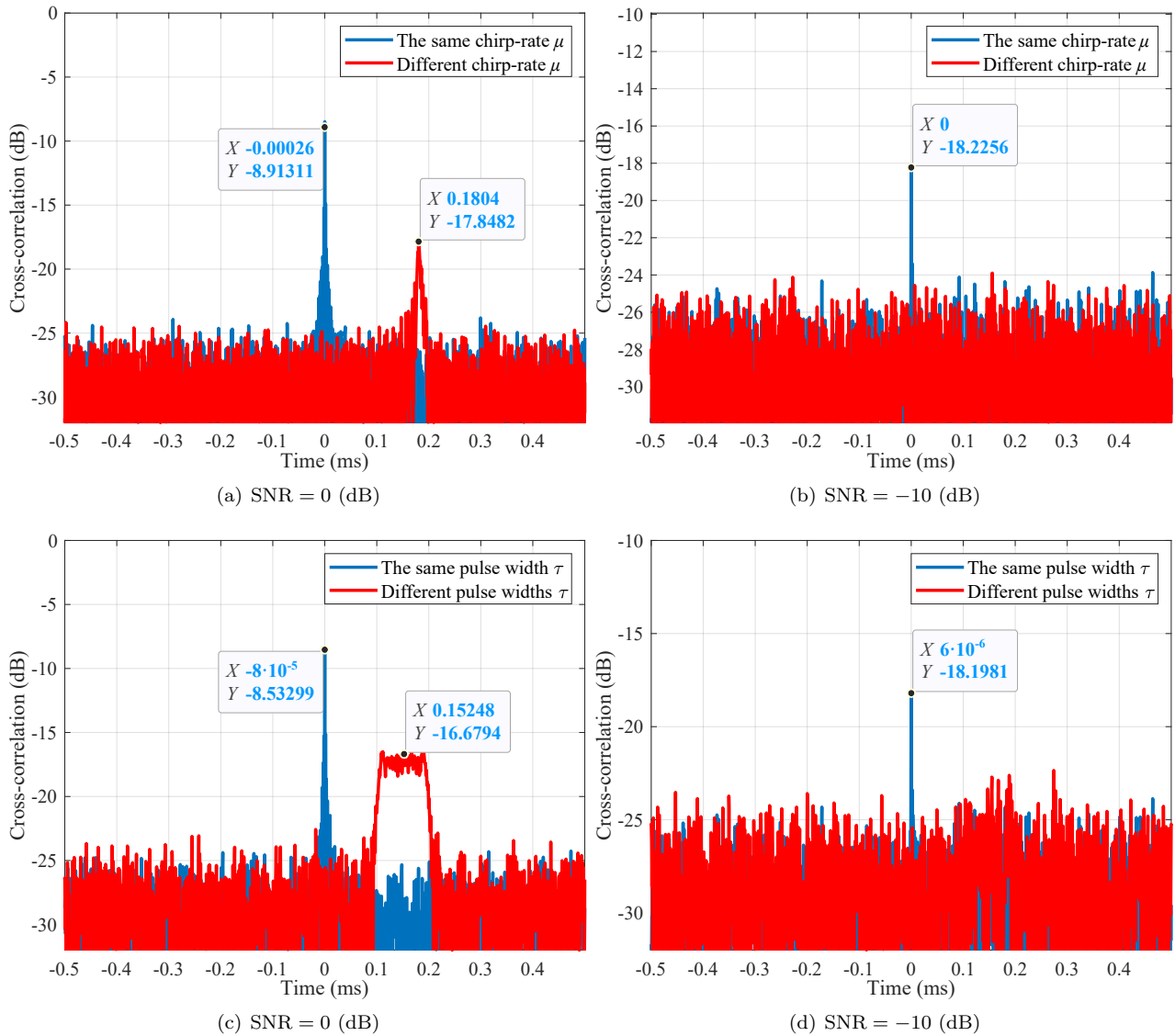
Fig. 2: CCF of between two signals at different levels of SNR: (a) SNR = 0 (dB), (b) SNR = -10 (dB) with different chirp-rate, (c) SNR = 0 (dB), (d) SNR = -10 (dB) with different pulse widths.
