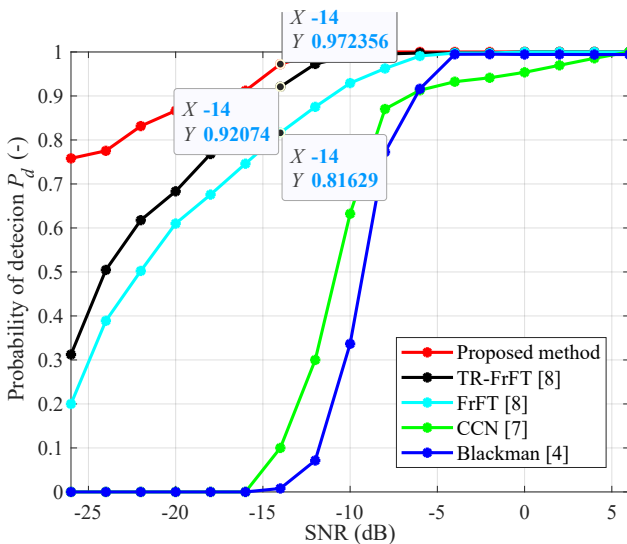
Fig. 9: Probability of detection of methods depends on SNR.
