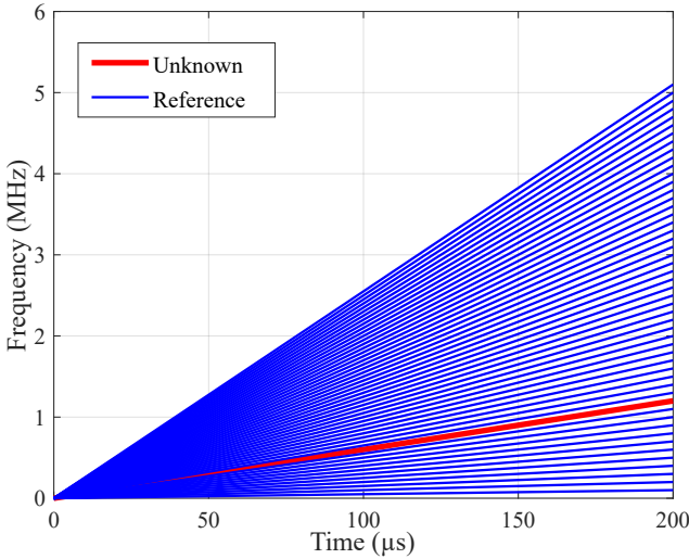
Fig. 3: Time-frequency characteristics of the unknown and reference LFM signals.
