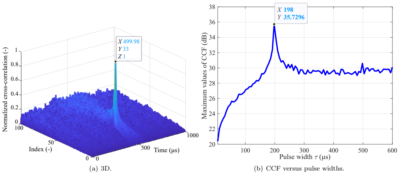
Fig. 5: CCF between unknown and second reference LFM signals: (a) 3D, (b) CCF versus pulse widths.
