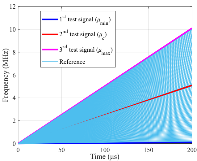
Fig. 6: Time-frequency characteristics of LFM signals.
