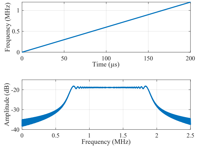
Fig. 1: Time-frequency characteristics and amplitude spectrum of chirp-up LFM signal.
