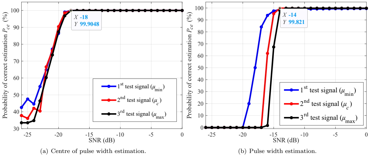
Fig. 8: Probability of correct estimation depends on SNR: (a) centre of pulse width estimation, (b) pulse width estimation.
