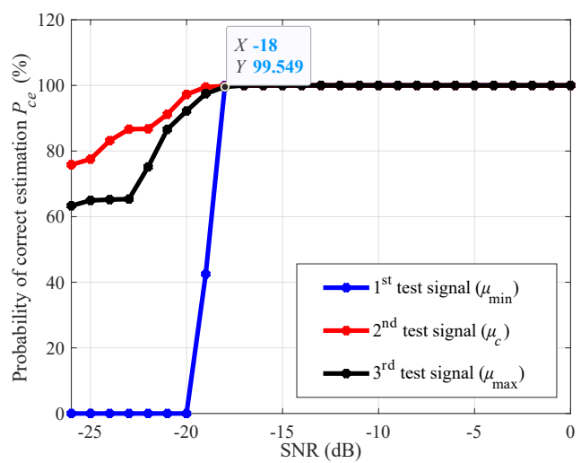
Fig. 7: Probability of correct estimation depends on SNR.
