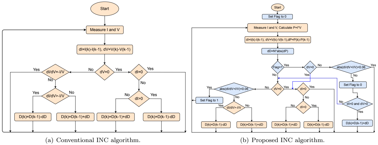
Fig. 4: Flowcharts of conventional and proposed INC algorithms.
