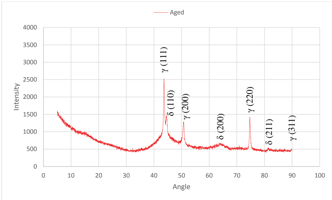
Figure 7: The XRD spectra of AM 304L stainless steel in (a) As-built material, (b) Aged sample
