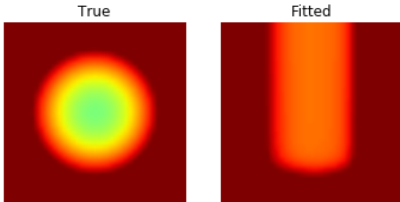
Figure A.3: Demonstration of our network architecture’s ability to create a function which is monotonic in one dimension and non-monotonic in another, even when the data does not meet those qualifications.
