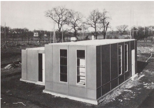
Figure 1: Stahlhaus during its construction. Source: Engelmann, Ch. and Schädlich, Ch. (1991). Die Bauhausbauten in Dessau . Berlin: Verlag für Bauwesen.
