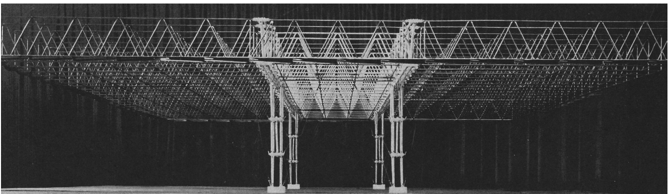
Figure 2: Model of Mobilar Structure System . Source: Arribas-Blanco, R. (2016). Jean Prouvé and Konrad Wachsmann. Two ways of using the scale model as a tool for projecting. Proyecto, Progreso, Arquitectura . 15, 56-69.
