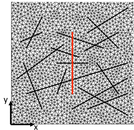
Figure 3: Considered domain with unstructured gridding. The black solid lines represent fracture while the red one represents wellbore.
