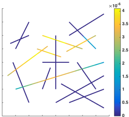
Figure 7: The increase in apertures at the end of 10 days of constant injection process (matrix permeability: 10^{-21} \text{ m}^3 ).
