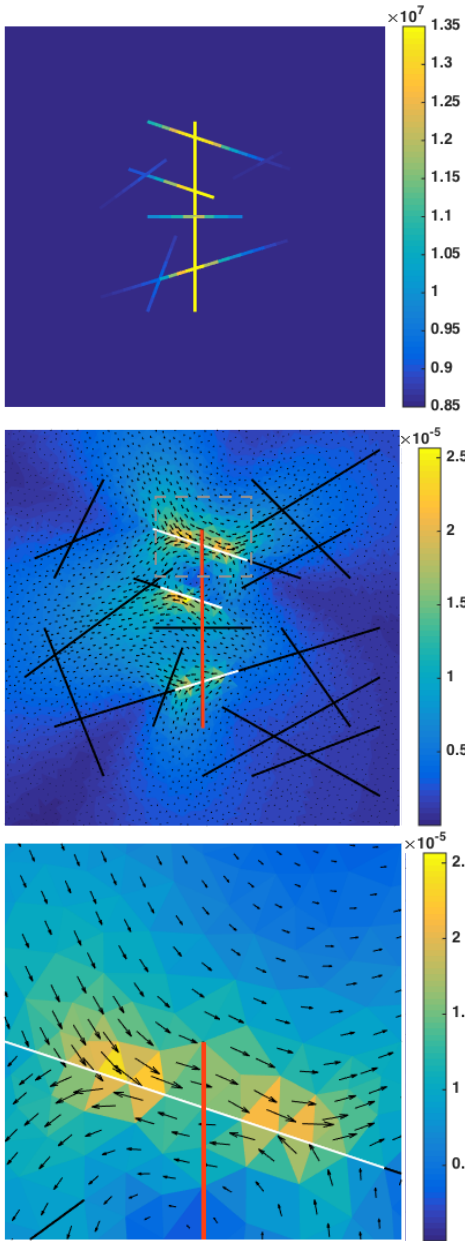
Figure 5: The pressure distribution (top) and induced displacement (middle) after 2000s. To have better inspection of the displacements, the bottom figure shows closer look of grey dashed lined area of the middle figure.
