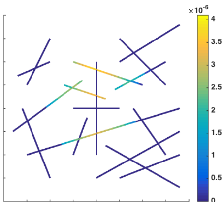
Figure 8: The increase in apertures at the end of 10 days constant injection process (matrix permeability: 10^{-20} \text{ m}^3 ).
