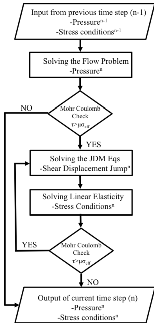
Figure 2: The solution strategy for each time step.
