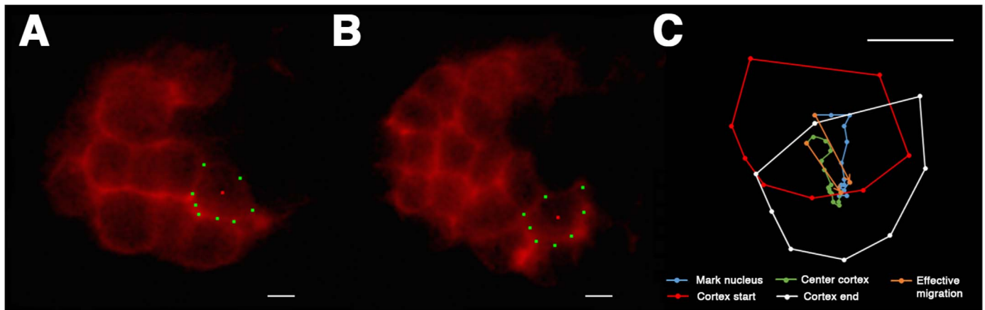
Fig. 4. Precision of the recording of cell position. (A) The cortex of the cell ABarapp of an otherwise wild-type embryo is highlighted with a Pmex-5::Lifeact::mKate2 transgene (SWG001) (Reymann et al., 2016) construct at the frame 175 of the recording. The green dots mark the shape of the cortex and the red dot the center of the cell, which we mark normally in the DIC recordings. (B) The end of the analysis of the cell at frame 188. The cell changes its shape constantly. (C) The red octagon represents the cortex at frame 175, the white octagon at frame 188. The eight positional marks are used to calculate the center of the cell, whose movement is shown by the 15 dots. The 15 dots show the marks of the visually tracked center. The corresponding marks deviate on average by 1.11 \pm 0.53 \mu\text{m} (mean \pm SD n = 15 ), which corresponds to 10% of the cell diameter at the 128-AB cell stage used for the analysis (scale bar 5 \mu\text{m} ).
