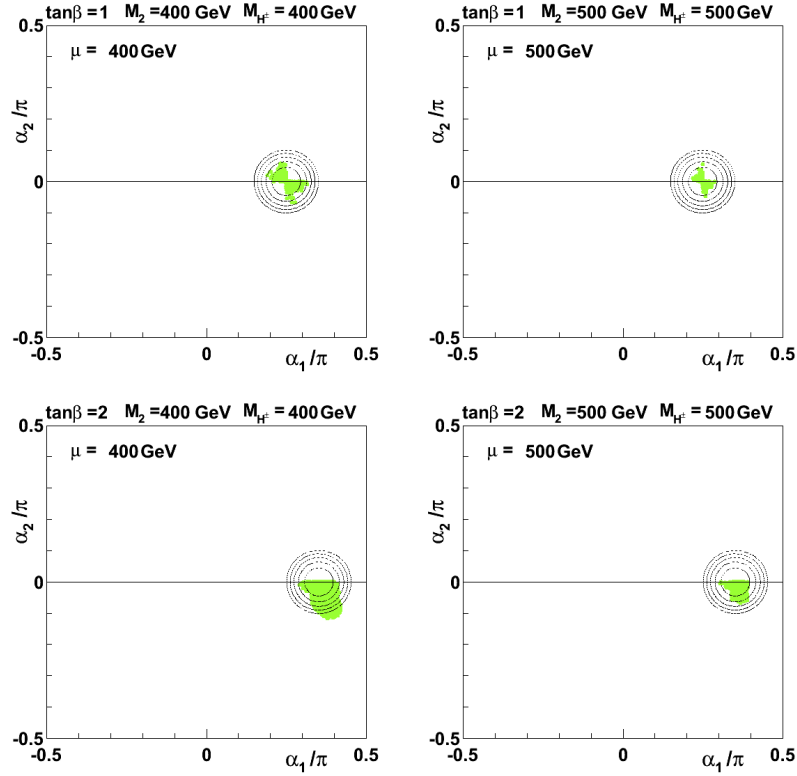
Figure 3: The H_1 SM (alignment) limit: Allowed regions in the \alpha_1 – \alpha_2 plane for the simplified model with \lambda_6 = \lambda_7 = 0 .
