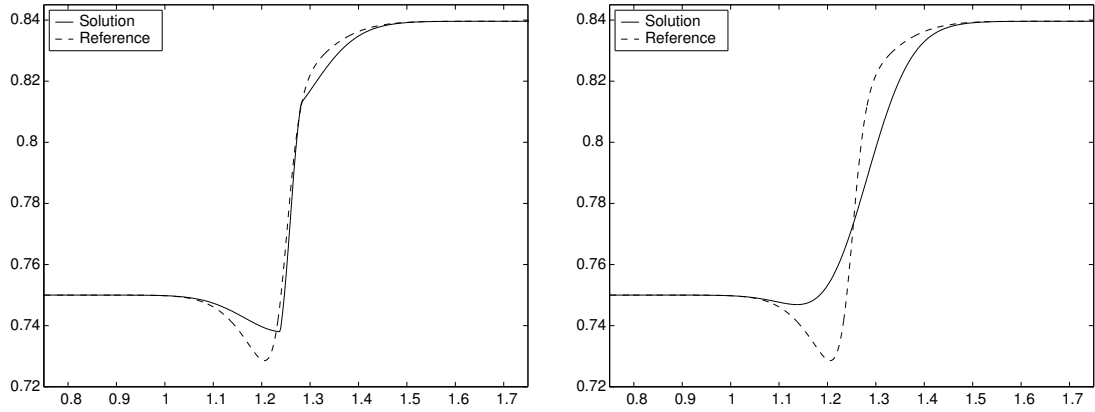
FIGURE 11. Example 3. Comparison of the s -component as a function of x for splitting solutions computed with two steps of COS (left) and OS (right).
