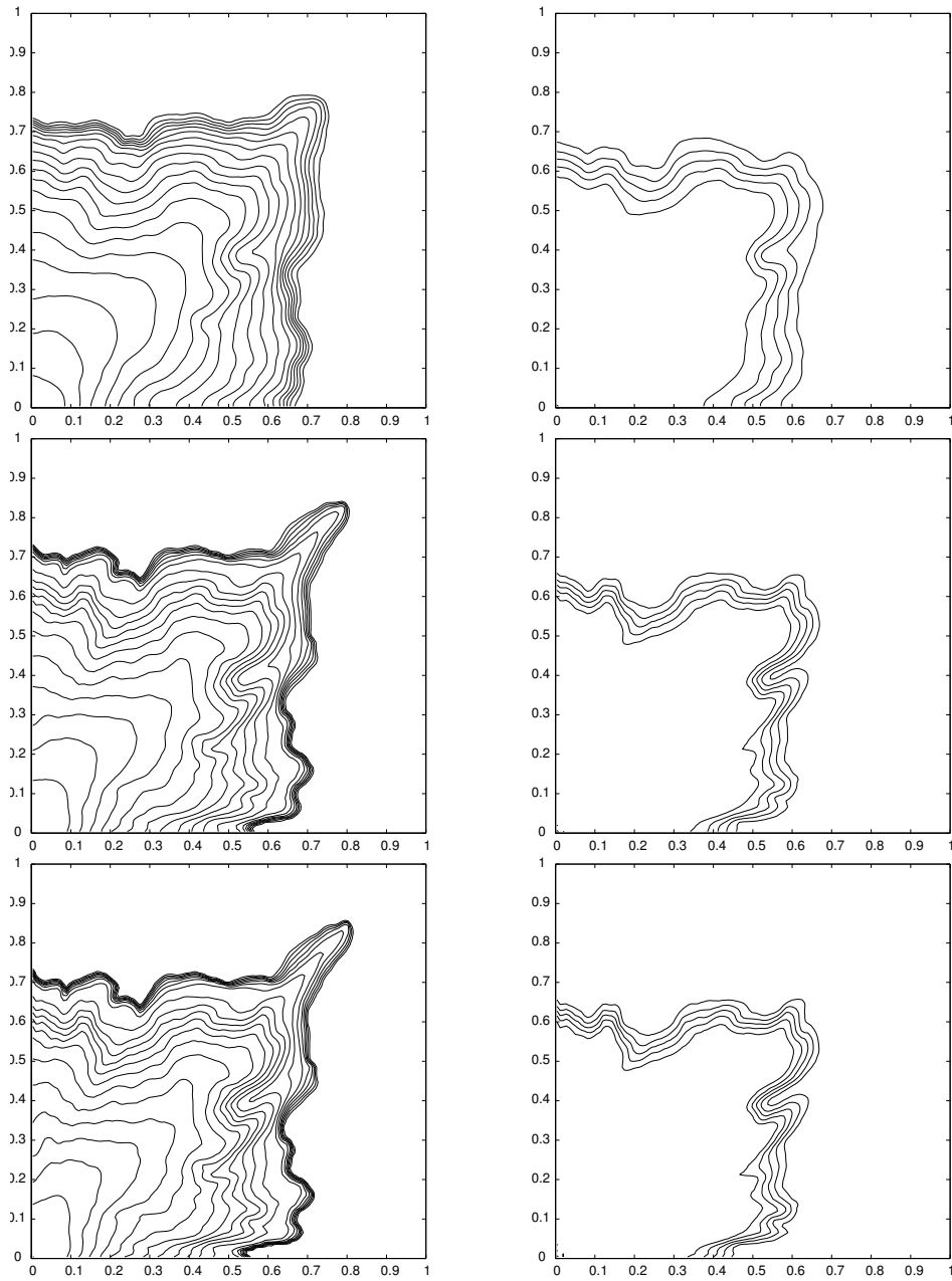
FIGURE 19. Example 2. Saturation and concentration profiles at time t = 0.3 computed on a 129 \times 129 grid. The diffusion coefficient is \varepsilon = 0.05, 0.005, \text{ and } 0.0005 from top to bottom.
