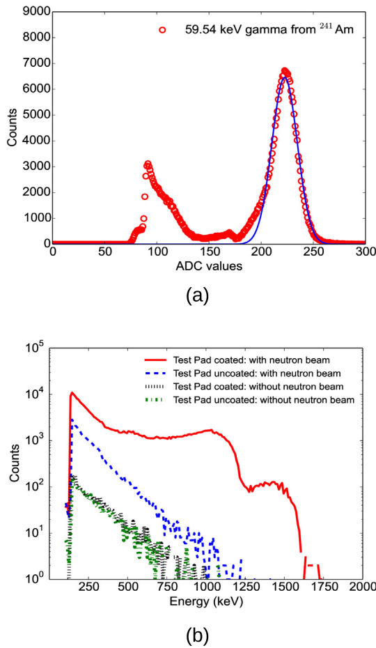
Fig. 3. (a) Energy spectrum obtained from a 59.54 keV gamma emitted from an ^{241}\text{Am} source for energy calibration purposes. The blue represents a Gaussian fit to the data, (b) Four energy spectra obtained from planar detector Test Pad: Two from the uncoated detector and two from in presence and absence of the neutron beam, two from the detector coated with enriched \text{B}_4\text{C} in presence and absence of the neutron beam respectively. (For interpretation of the references to colour in this figure legend, the reader is referred to the web version of this article.)
