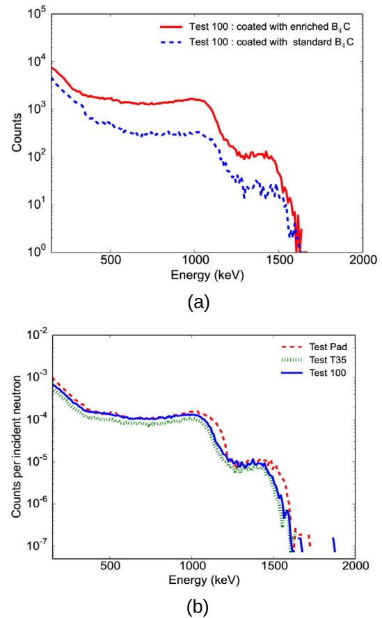
Fig. 4. Experimental results: (a) Effect of ^{10}\text{B} enrichment: energy spectra from detectors patterned with a 2D array of inverse pyramids (Test 100) and coated with either natural or enriched \text{B}_4\text{C} . (b) Effect of patterning: energy spectra obtained from the planar detector Test Pad, the detector patterned with an 1D array of pyramids (Test T35) and the detector patterned with a 2D array of pyramids (Test 100), all coated with enriched \text{B}_4\text{C} .
