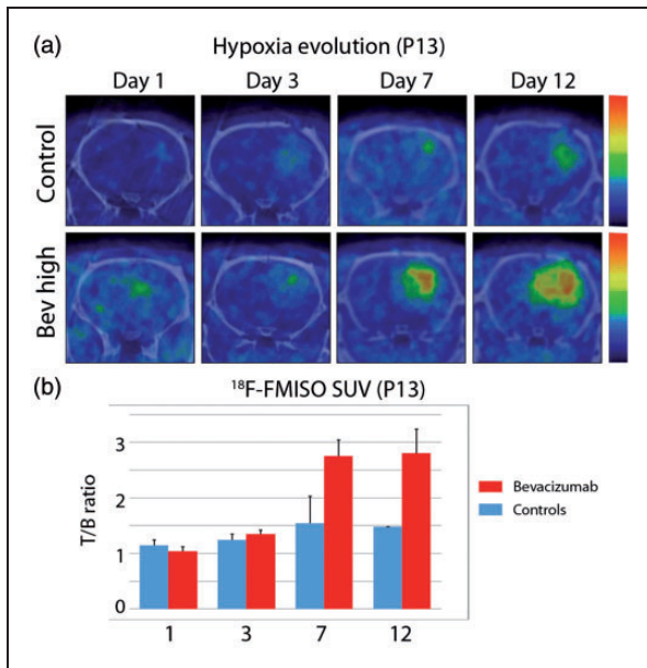
Figure 5. Tumoural hypoxia evolution. (a) Representative images of the longitudinal changes in hypoxia for P13 animals, assessed 18 F-FMISO PET, illustrate the high increased uptake of this tracer following treatment with bevacizumab (high dose) compared to the controls. SUV in arbitrary units. (b) Quantification of the ratio of 18 F-FMISO standard uptake value (SUV) in tumour versus brain confirms these findings. The following numbers of animals were used (Controls: 4, Bev 10 mg/kg: 4). (Scale bars: SEM).
