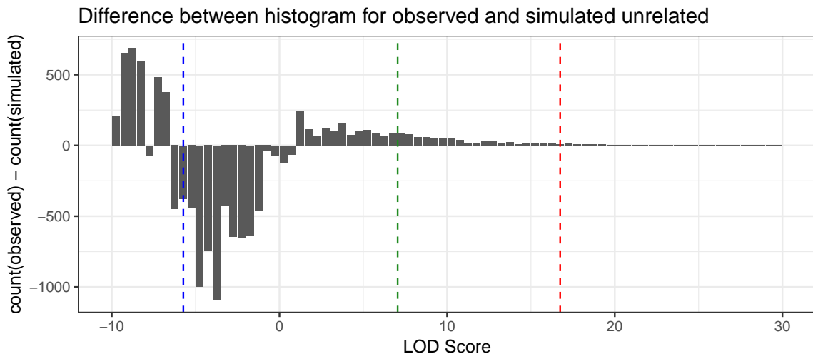
Figure 5.3: Difference between the counts in each bin for observed values and simulated values for unrelated pairs. The observed distribution is skewed left of the expected distribution, and has a heavy right tail. Blue, green and red lines are means from expected distributions (fig. 5.1).
