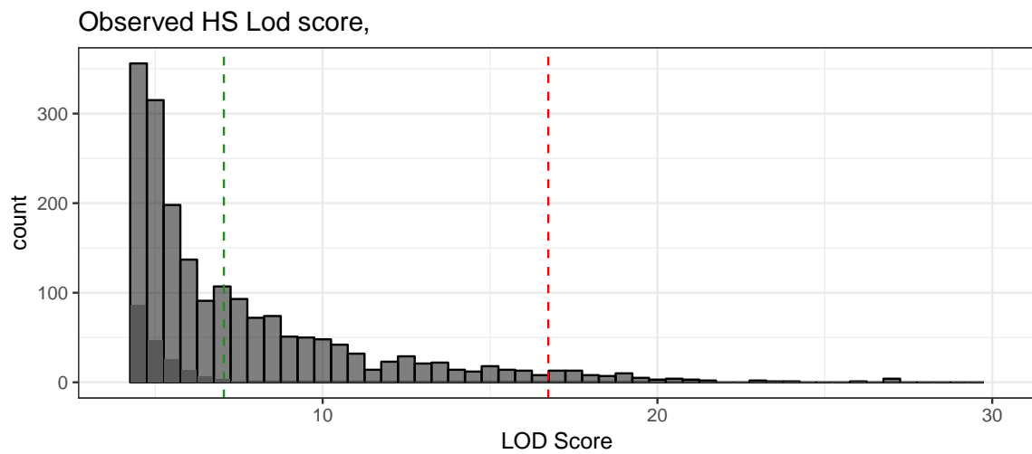
Figure 5.4: Right tail of histogram of observed pairwise LOD scores. The darker columns to the left is expected number of unrelated from Gaussian approximation of unrelated LOD (the solid line in fig. 5.1)
