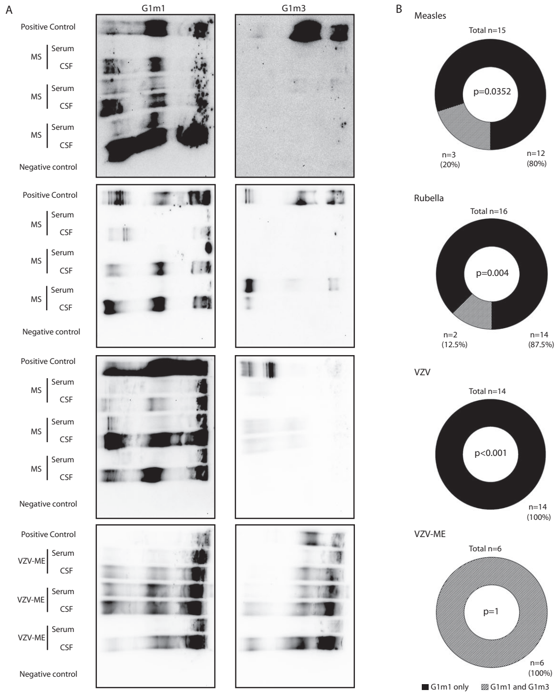
Figure 1. Intrathecal synthesis of IgG1 against measles, rubella and varicella zoster virus (VZV) shows G1m1 allotype predominance in MS patients and an even distribution in controls with VZV meningoencephalitis (VZV-ME). (A) The three upper panels show representative isoelectric focusing and affinity blotting against measles, rubella and VZV, determining IgG1 synthesis of G1m1 and G1m3 allotypes in three G1m1/G1m3 heterozygous MS patients. CSF samples from homozygous MS patients with virus-specific intrathecal synthesis were used as positive and negative controls. The bottom panel shows the results from three representative controls with VZV-ME after affinity blotting against VZV. (B) Isoelectric focusing and affinity blotting was performed on paired CSF and serum samples of G1m1/G1m3 heterozygous MS patients to determine G1m1 allotypes of intrathecally synthesized antibodies against measles, rubella and VZV. The same procedure was used to determine the G1m1 allotypes of intrathecally synthesized antibodies against VZV in G1m1/G1m3 heterozygous controls with VZV meningoencephalitis. The intrathecal synthesis of IgG1 of the G1m1 allotype alone was compared to that of IgG1 of both allotypes using Binomial test.
