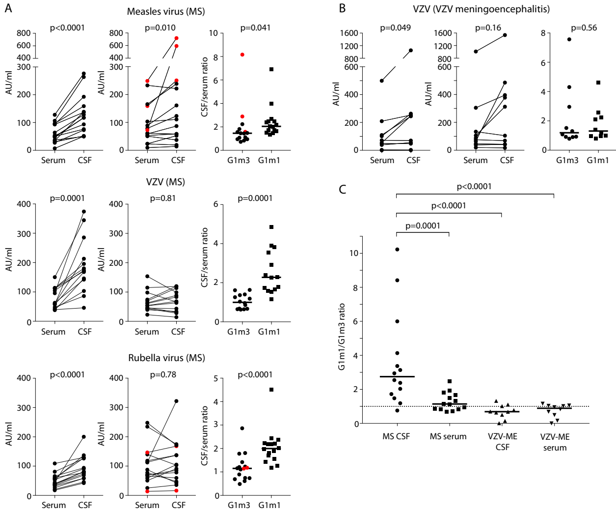
Figure 2. Anti-viral antibodies of the G1m1 allotype are enriched in cerebrospinal fluid (CSF) of MS compared to serum, and compared to CSF and serum of controls with varicella zoster virus meningoencephalitis (VZV-ME). (A) Measles-, rubella-, and VZV-specific G1m3 and G1m1 antibodies were quantified in paired serum and CSF samples of MS patients using ELISA, and the CSF:serum ratios were estimated. The bars depict the median values. Comparisons were made using the Wilcoxon signed-rank test. Exceptions displaying G1m3 usage according to isoelectric focusing and affinity blotting are marked in red. (B) VZV-specific G1m3 and G1m1 antibodies were quantified in paired serum and CSF samples of VZV-ME controls using ELISA, and the CSF:serum ratios were estimated. The bars depict the median values. Comparisons were made using the Wilcoxon signed-rank test. (C) G1m1/G1m3 ratios of VZV-specific antibodies in MS and VZV-ME samples of CSF and serum. The bars correspond to the median values. Statistical significance was established using Kruskal-Wallis test on all groups, Wilcoxon signed-rank test comparing patient CSF and serum, and Mann-Whitney U test comparing patients and controls.
