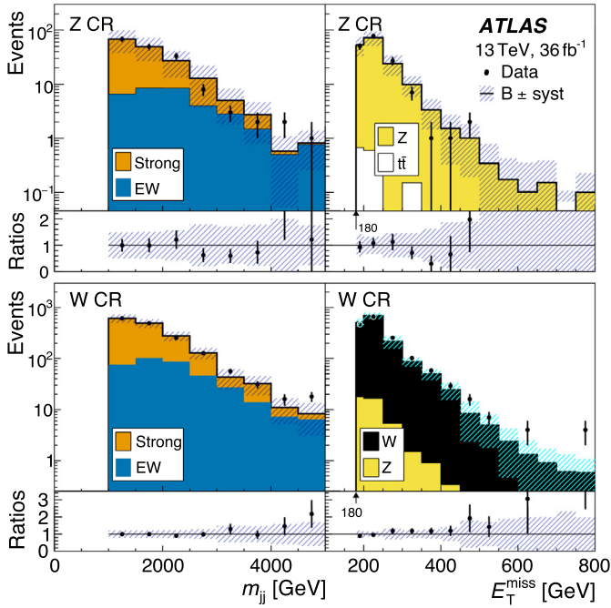
Fig. 2. Distribution of event yields in the Z (top) and W (bottom) control regions. The postfit normalizations for m_{jj} (left) and E_T^{miss} (right) are summed over the subsamples. The E_T^{miss} distributions start at 180 GeV as indicated. The observed data N (dots) are superimposed on the sum of the backgrounds B (stacked histogram with shaded systematic uncertainty bands). The breakdown of the B is given in the lower left box in each panel. The bottom panels show the ratios of N to B with the systematic uncertainty band shown on the line at 1. The “other,” as listed in Table 1, contribute a few events at low values of m_{jj} and E_T^{miss} , and are omitted. The last bin in each plot contains the overflow.
