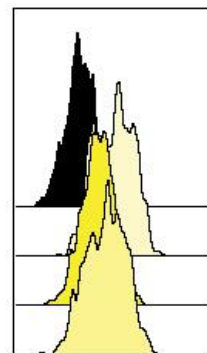
Fig.30: Histogram
