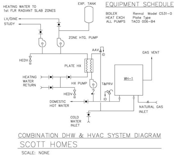
Figure 4 – Scott Homes, combo space/DHW system mechanical drawing
