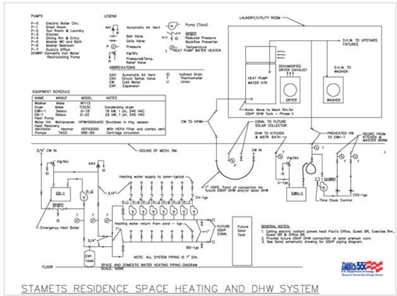
Figure 8 – Stamets Residence, Mechanical System Drawing (noting GSHP installation of fall 2008)
