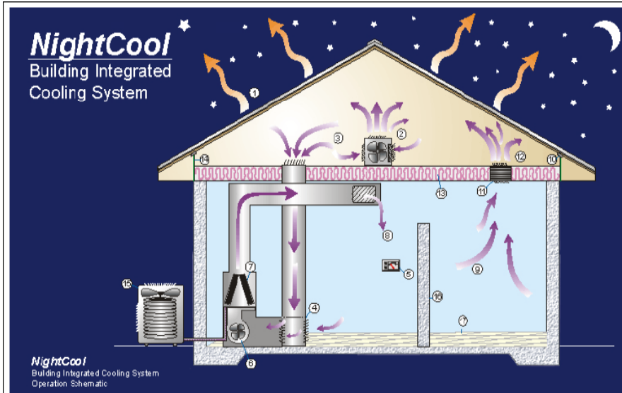
Figure I- 8 Schematic of NightCool concept
