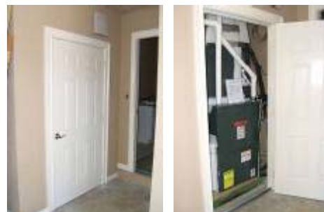
Figure 3- 11 Exterior walls around air handler isolate closet from garage, create valuable conditioned square footage.
