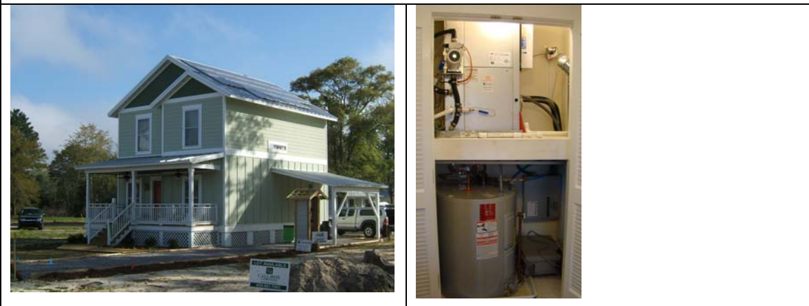
Figure I- 11. The NZEH by Stalwart Built Homes (l) with its geothermal heat pump with heat recovery DHW (r).
