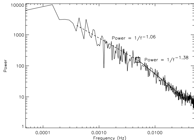
Fig. 4. Sum of power spectra of our four XMM/EPIC pn observations over 0.8–10 keV of \gamma Cas. The binning in time over 10 s prevents the spectrum from being followed out to its white noise component. Regression lines are drawn with slopes noted through two frequency ranges. A break in the slopes is noted by a square symbol at a frequency of 0.005 Hz.
