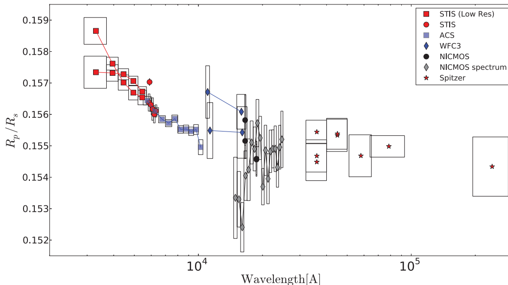
Figure 9. Transmission spectrum data, with data sets and visits indicated separately. Lines connect values obtained at the same time with the same instrument.
