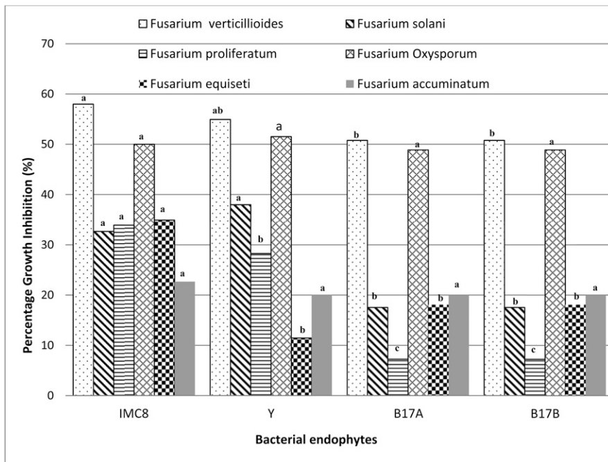
Fig. 1. The performance of bacterial endophytes in suppressing mycelial growth of diverse Fusarium species in dual cultures exhibiting their potential as biological control agents. Bacterial endophytes IMC8 ( Bacillus thuringiensis ); Y ( B. thuringiensis ); B17A ( Stenotrophomonas sp.); and B17B ( Serratia sp.). Different letters in each fungal pathogen (column patterns) indicate statistical differences at P = 0.05 according to SAS Prolog analysis.
