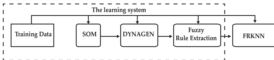
Figure 2. Modelo FRKNN (Laha, 2007)
