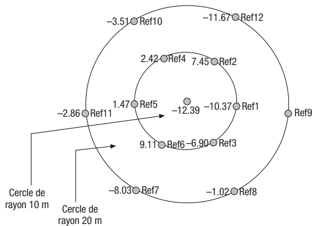
Figure 7. Erosion and deposition rates ( \text{tha}^{-1} \text{yr}^{-1} ) estimated by using distribution profile model for all sampling points; negative values are expressing erosion while positive are deposition.
