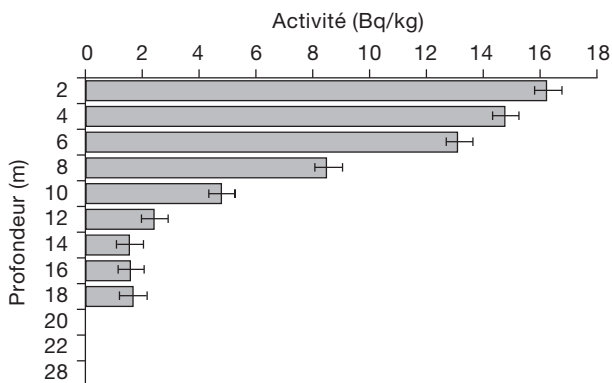
Figure 6. Depth distribution profile of ^{137}\text{Cs} in cork oak forest soil.
