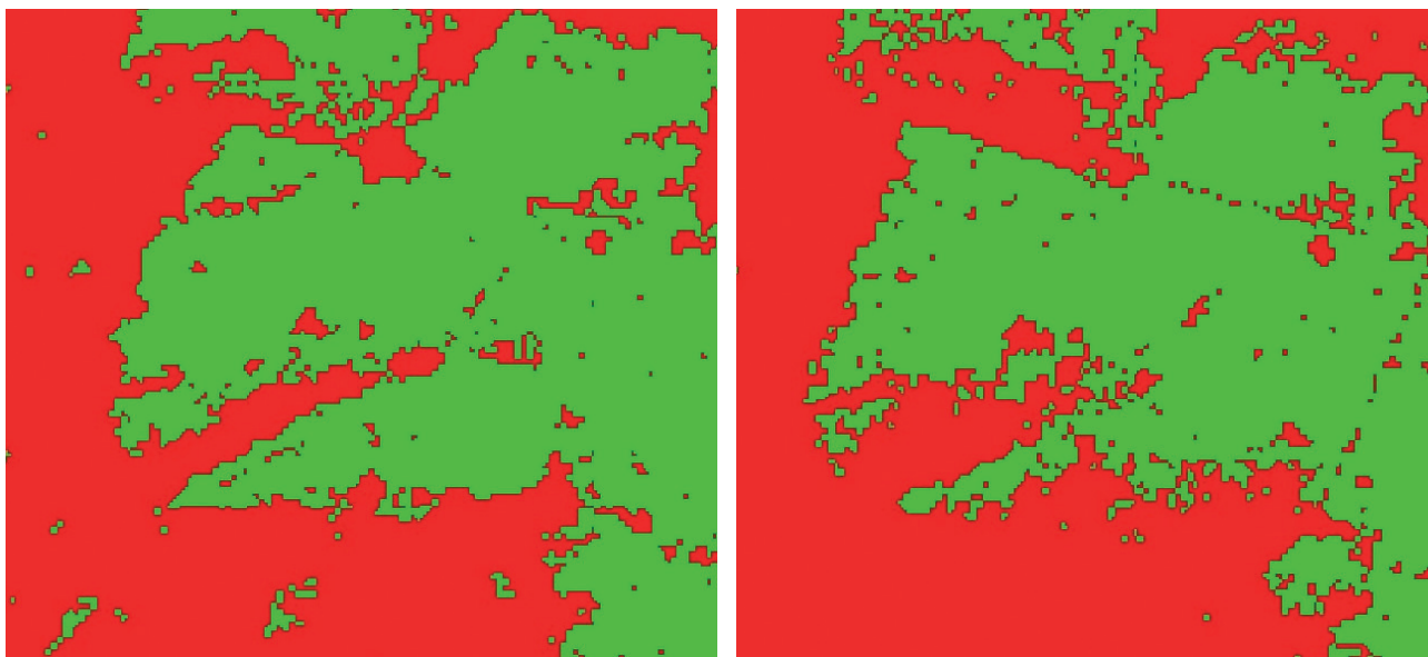
Figure 5. The borders of the Sidi Azzouz forest in 1987 and 2003. From: Aster images.
