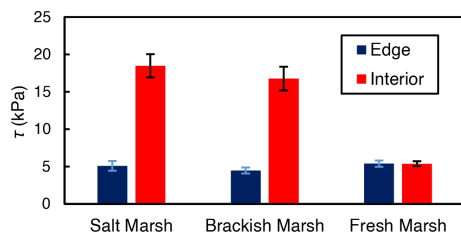
Figure 4. Average shear strength ( \tau ) values for the marsh edge and the interior locations. The salt marsh locations are Goodwin Islands and Catlett Islands, the brackish marsh location is Taskinas Creek, and the freshwater marsh locations are Sweet Hall Marsh and the Pamunkey Indian Reservation. Each column represents the depth-averaged shear strength for the upper 30 cm of soil of each marsh type, and error bars represent the standard error of 10 replicate shear strength profiles for each marsh type.
