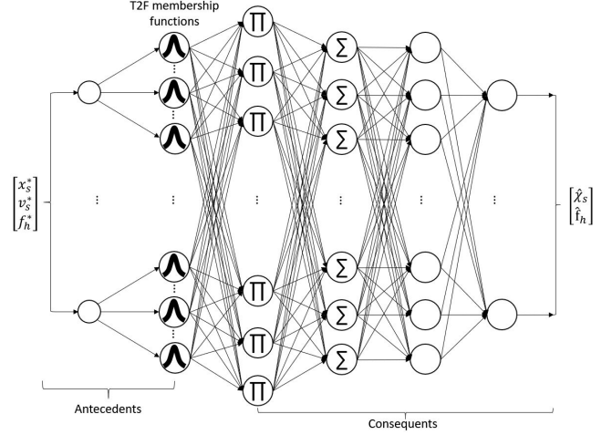
Fig. 4. Structure of the IT2FNN models.
