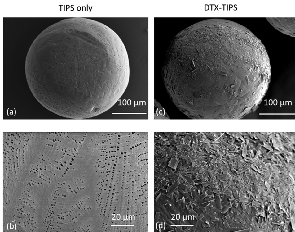
Figure 1. Ultrastructural imaging of 10% (w/v) PLGA TIPS microparticles. a) Unloaded control PLGA TIPS microparticle. b) Higher magnification of unloaded control PLGA TIPS microparticle with the porous surface features of the microparticles visible. c) PLGA DTX-TIPS microparticle. d) Higher magnification of PLGA DTX-TIPS microparticle with precipitated DTX visible on the surface.
