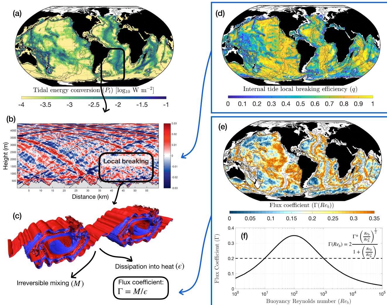
Figure 1. (a) Energy conversion into internal tides, reconstructed from Vic et al. (2019). (b) Generation of internal tides over rough topography (the panel shows internal tide velocities [m/s] from numerical simulations, from Nikurashin and Legg, 2011). A fraction of the power in the generated waves, (1 - q) , radiates away from the generation region, while the remaining fraction q is converted locally. (c) (from Mashayek, Caulfield, & Peltier, 2017) From each wave breaking event, part of the energy in the generated turbulence is converted into irreversible mixing (with rate \mathcal{M} ), while the rest is viscously dissipated (with rate \epsilon ), such that \Gamma = \mathcal{M}/\epsilon . (d) Internal tide local breaking efficiency q(x, y) , reconstructed from Vic et al. (2019). (e) Flux coefficient \Gamma(Re_b) at 3,500 m, using (f) the parameterization of Mashayek, Salehipour, et al. (2017). The maximum flux coefficient ( \Gamma^* = 0.35 ) occurs at Re_b^* = 100 ; both values fall within the bound reported in Mashayek, Salehipour, et al. (2017).
