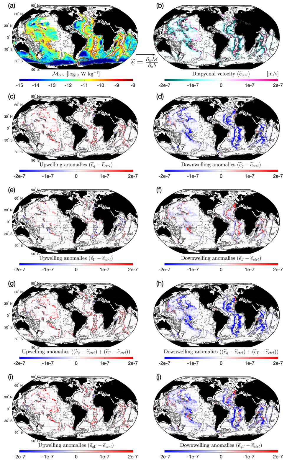
Figure 2. (a) Diapycnal mixing (log scale) over the neutral density surface \gamma^n = 28.1 for case ( ctrl ), that is, q = 0.3 , \Gamma = 0.2 . All the following panels are on the same neutral density surface. (b) Diapycnal velocity \tilde{e} for case ( ctrl ), with negative velocities (dark cyan) indicating downwelling and positive velocities (magenta) indicating upwelling. Panels (c) and (d), (e) and (f), and (i) and (j) show differences in upwelling (left column) and downwelling (right column) between the different cases and case ( ctrl ). Panels (g) and (h) show the sum of the anomalies of case (q) and case ( \Gamma ) with respect to case ( ctrl ).
