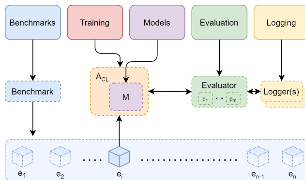
Figure 1: Operational representation of Avalanche with its main modules (top), the main object instances (middle) and the generated stream of data (bottom). A Benchmark generates a stream of experiences e_i which are sequentially accessible by the continual learning algorithm A_{CL} with its internal model M . The Evaluator object directly interacting with the algorithm provides a unified interface to control and compute several performance metrics ( p_i ), delegating results logging to the Logger(s) objects.
