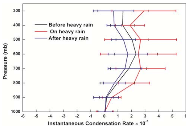
Fig. 6 — Vertical profile of condensation rate over Chennai before, on and after the heavy rainfall events during the northeast monsoon of 2001 to 2015.
