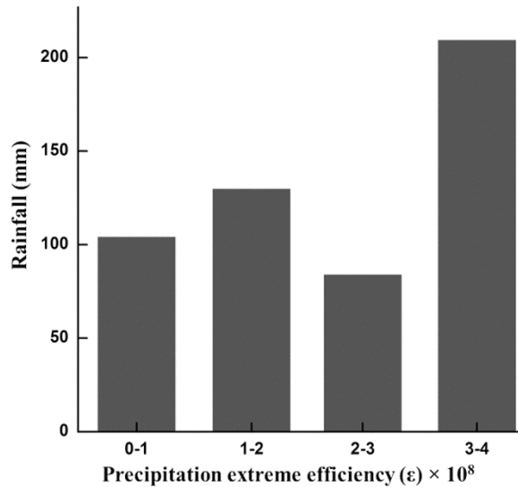
Fig. 8 — Precipitation extreme efficiency ( \epsilon ) during the heavy rainfall events over Chennai.
