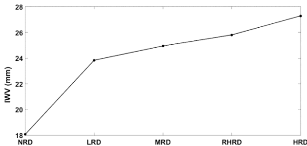
Fig. 2 — Scaling of IWV with the non-rainy, light, moderate, rather heavy and heavy rainy days over Chennai during NE monsoon of 2001 to 2015
