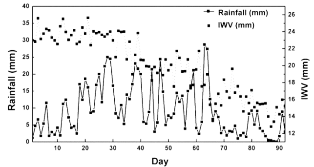
Fig. 1 — Mean daily rainfall and IWV over Chennai during NE monsoon of 2001 to 2015.
