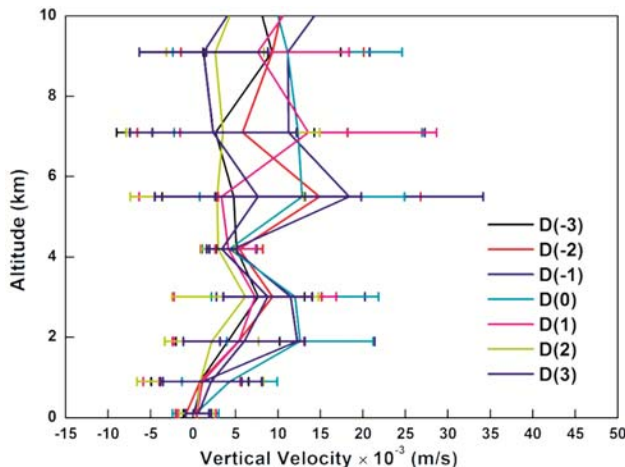
Fig. 5 — Averaged vertical profile of vertical velocity (m/sec) before, on and after the heavy rainfall events over Chennai.
