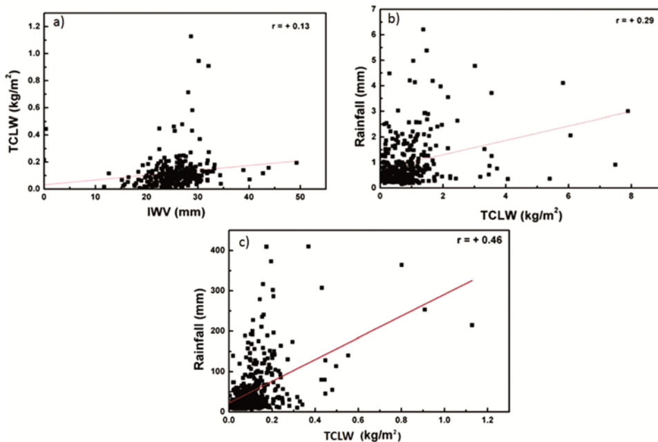
Fig. 3 — Correlation between a) TCLW and IWV, b) TCLW and rainfall and c) TCLW and rainfall of two consecutive days.
