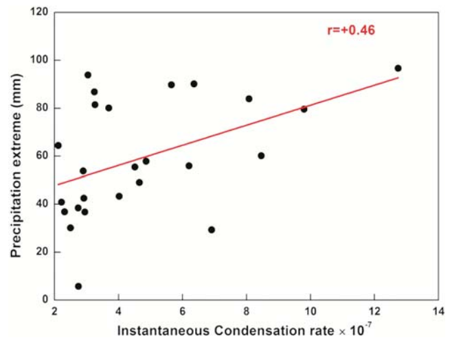
Fig. 7 — Scatter plot of integrated instantaneous condensation rate and integrated precipitation extreme over Chennai during heavy rainfall events.
