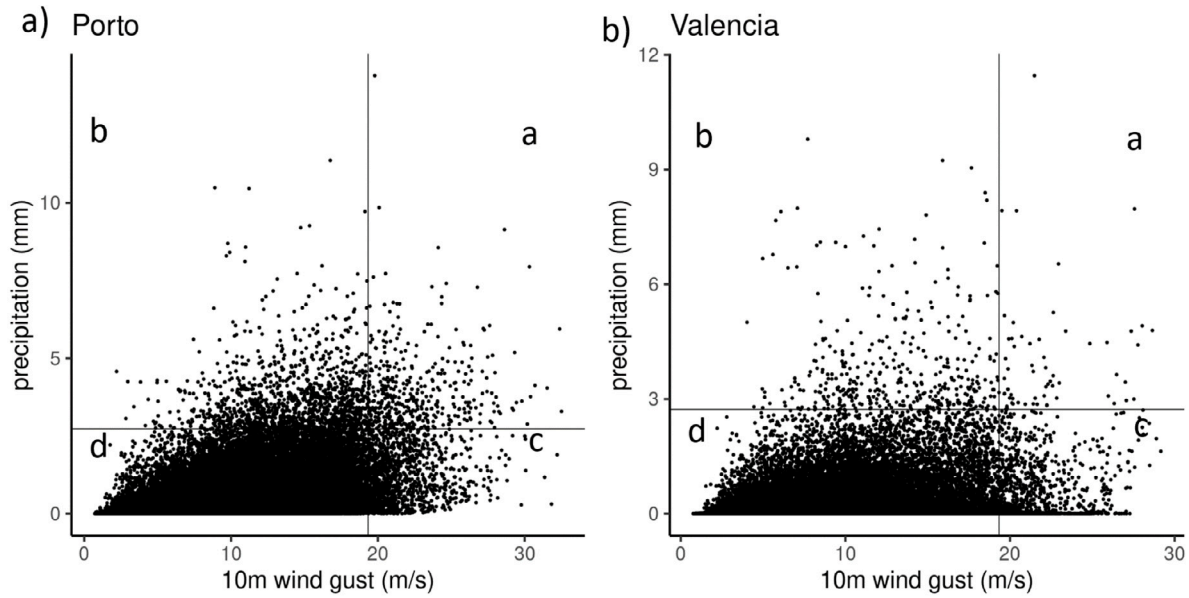
Fig. 1. Hourly 10 m wind gust and precipitation for (a) Porto and (b) Valencia, with horizontal and vertical lines at the 0.99 quantile for precipitation and wind respectively. a, b, c and d represent the four different quadrants of the graph. Quadrant a includes the extreme co-occurring, b extreme precipitation, c extreme wind and d non-extreme hourly events.
