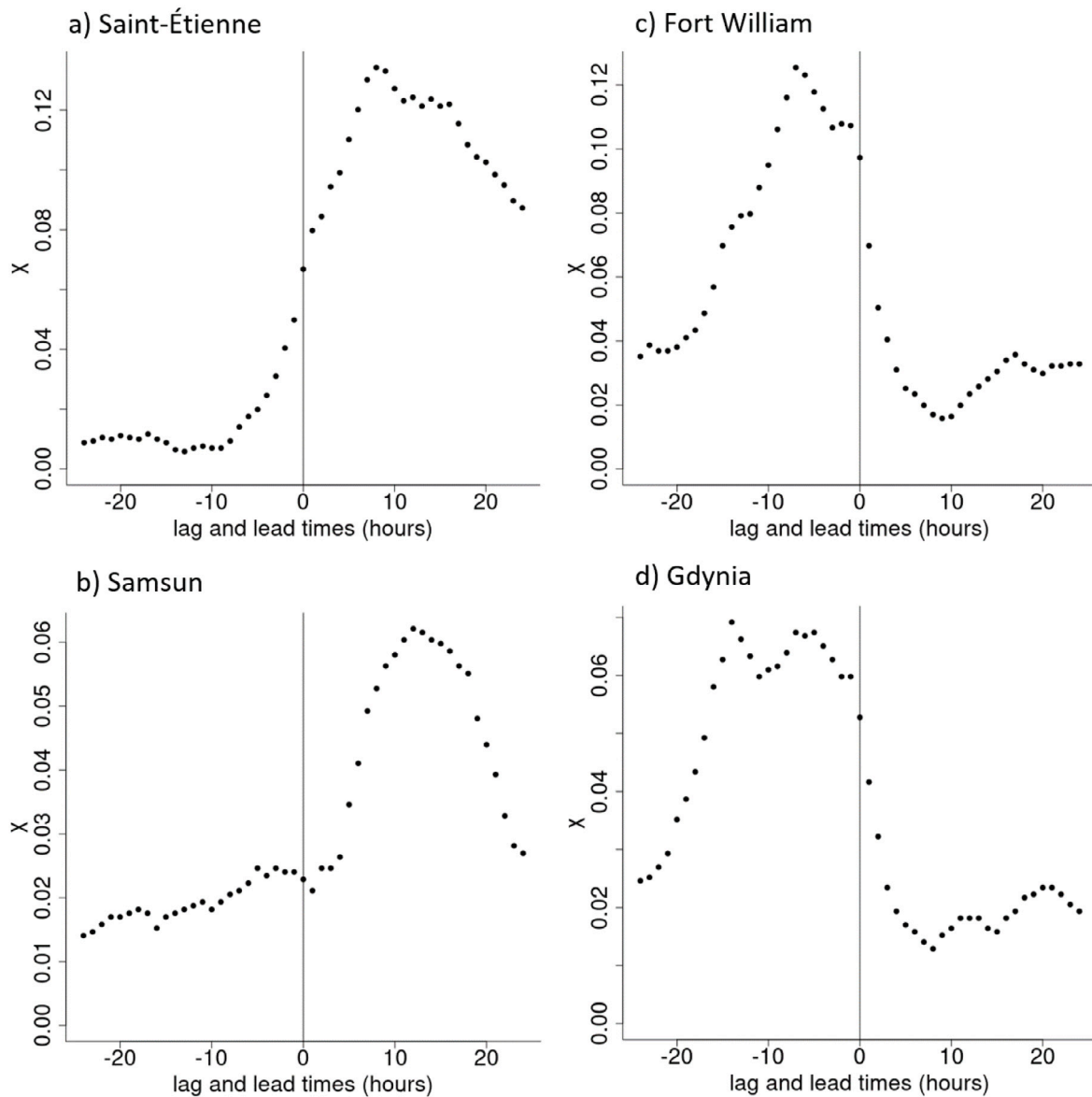
Fig. 8. \chi values for each 24 h lag and lead time for (a) Saint-Étienne, (b) Samsun, (c) Fort William and (d) Gdynia. Positive hours are when the largest \chi is given when the extreme wind gusts are occurring before the precipitation extremes and the negative hours are when the largest \chi is given when the precipitation extremes are occurring before the wind gust extremes.
