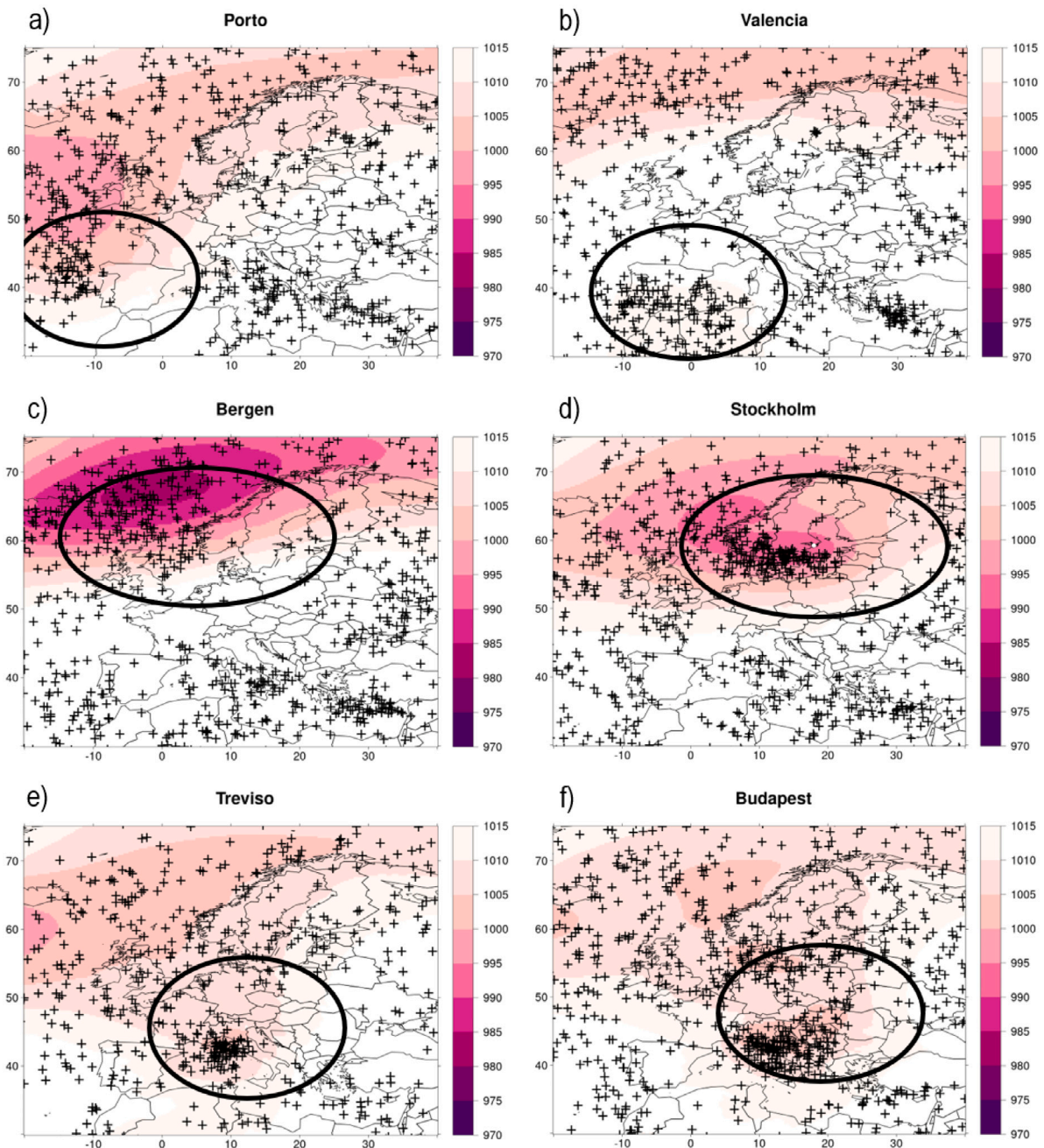
Fig. 11. As Fig. 10 but for the extreme precipitation events.
