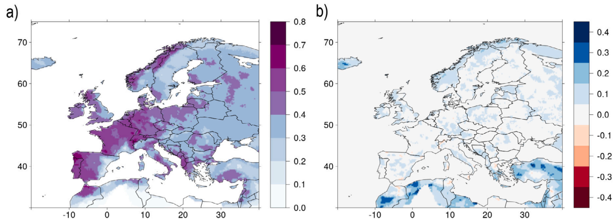
Fig. 6. (a) Extremal dependency, \chi , map for 80th percentile extremes from the ERA5/E-OBS dataset. (b) Difference in \chi between the ERA5/E-OBS and ERA5 datasets. A positive (blue) value indicates that the ERA5 dataset has a larger value of \chi . (For interpretation of the references to colour in this figure legend, the reader is referred to the web version of this article.)
