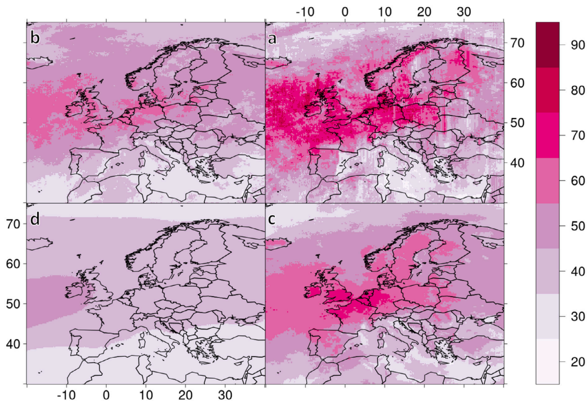
Fig. 15. The mean speed (km/h) of cyclones given the 6 hourly event sets a, b, c and d. Where a are the extreme co-occurring, b extreme precipitation, c extreme wind and d non-extreme 6 hourly events.
