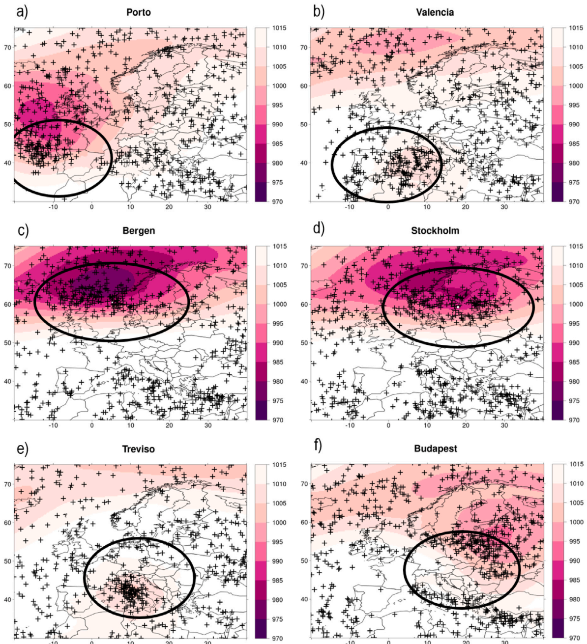
Fig. 12. As Fig. 10 but for the extreme wind events.
