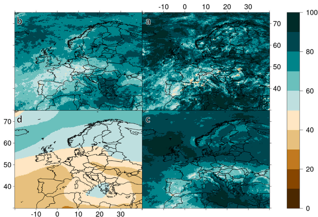
Fig. 9. Estimates of the probability of the presence of a cyclone given the 6 hourly event sets a, b, c and d. Where a are the percentages of extreme co-occurring, b extreme rain, c extreme wind and d non-extreme 6 hourly events. A cyclone is counted for a gridpoint if the gridpoints event occurs at the same 6 hourly timestamp and is within 1110 km from the cyclone tracks centre.
