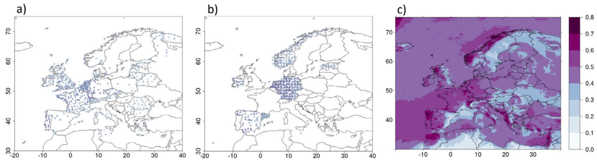
Fig. 4. Extremal dependency, \chi , maps for 80th percentile extremes from the (a) GSOD, (b) ECA, (c) ERA5 datasets.
