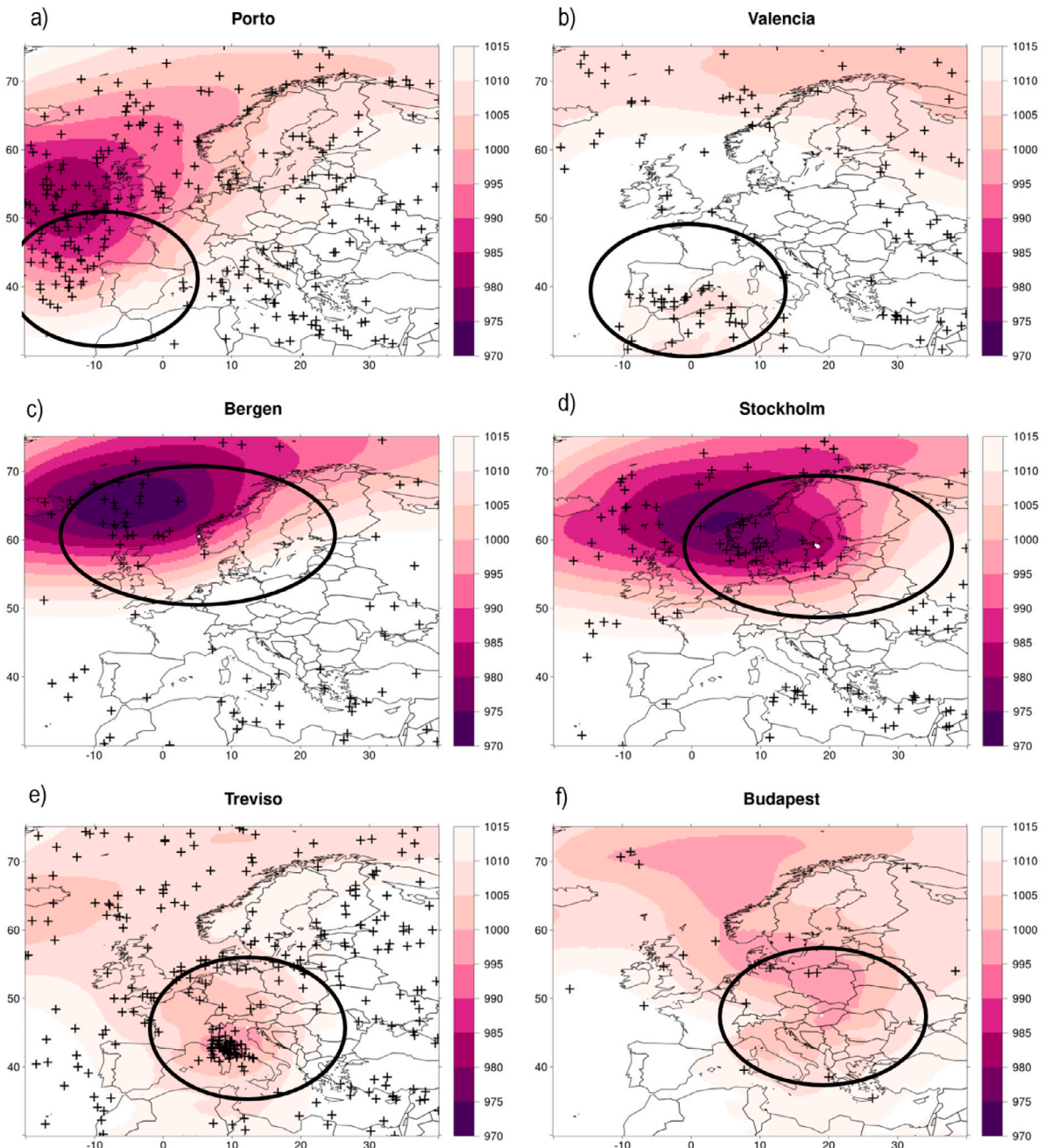
Fig. 10. Average MSLP plots for the extreme co-occurring events at locations (a) Porto, (b) Valencia, (c) Bergen, (d) Stockholm, (e) Treviso and (f) Budapest. These locations are selected due to their very low or very high \chi values. Crosses are the positions of cyclones identified by TRACK at the time of the extreme co-occurring events. Black circles indicate the approximate search regions.
