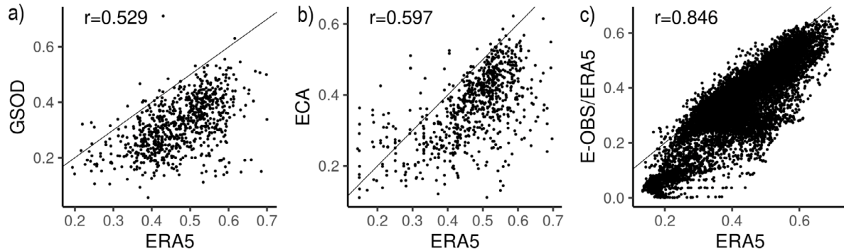
Fig. 5. Comparison between (a) GSOD and ERA5, (b) ECA and ERA5 to the nearest ERA5 grid box and (c) E-OBS/ERA5 and ERA5 \chi values, with corresponding correlation coefficients, r = 0.529 , r = 0.597 , and r = 0.846 . \chi values of 0 (over the sea) from the E-OBS/ERA5 dataset have been removed.
