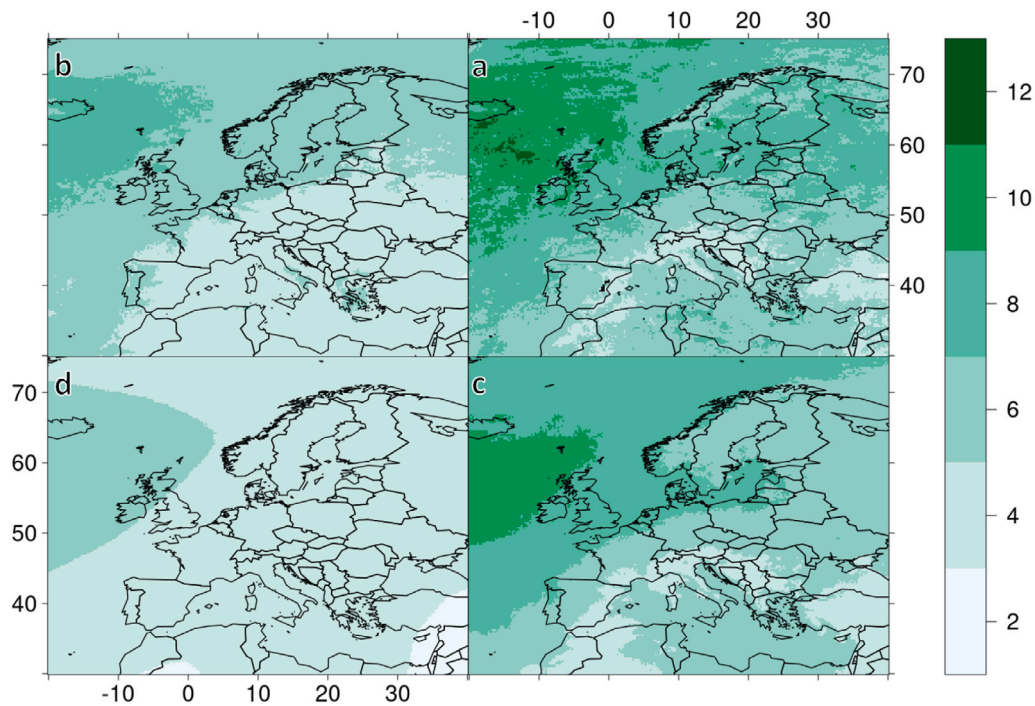
Fig. 13. The mean vorticity (rad/s) of cyclones given the 6 hourly event sets a, b, c and d. Where a are the extreme co-occurring, b extreme precipitation, c extreme wind and d non-extreme 6 hourly events. These panels indicate the relative difference in intensity to the local average intensity.
