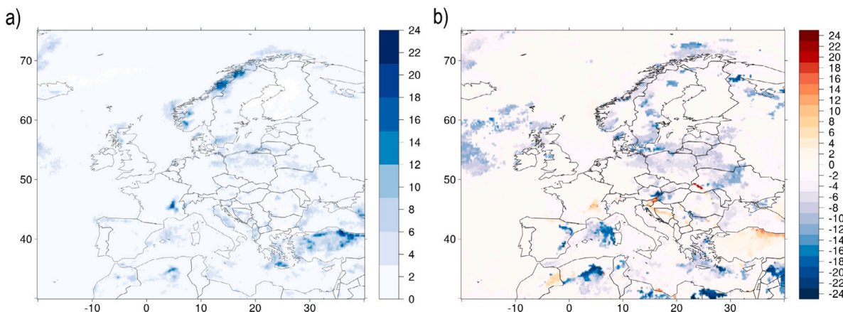
Fig. 7. (a) Percentage \chi increases when allowing up to a 24 h lag or lead between the precipitation and wind extremes for Europe. High percentages show regions where the highest \chi does not occur when extreme precipitation and wind occur within the same hour. (b) 24 h lag and lead times when \chi is at maximum. Red values indicate where wind gust extremes are arriving before precipitation extremes to give the largest \chi , white values where both extreme wind and precipitation arrive within the same hour to give the largest \chi and blue values where precipitation extremes are arriving before wind gust extremes to give the largest \chi . (For interpretation of the references to colour in this figure legend, the reader is referred to the web version of this article.)
