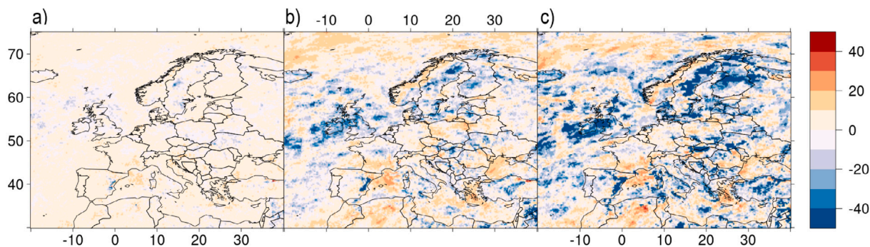
Fig. 3. Percentage difference, (\text{accumulated} - \text{hourly}) / ((\text{accumulated} + \text{hourly}) / 2) \times 100 , between hourly and (a) 6, (b) 24 and (c) 48 hourly \chi values. Areas of red represent where the accumulated periods give higher \chi values and areas of blue represent where the hourly period gives higher \chi values. (For interpretation of the references to colour in this figure legend, the reader is referred to the web version of this article.)
