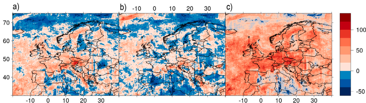
Fig. 16. The percentage change, ((u_a - u_b)/u_b) \times 100 , between event set a's mean speed ( u_a ) of a cyclone and (a) b ( u_b ), (b) c ( u_c ) and (c) d ( u_d ).
