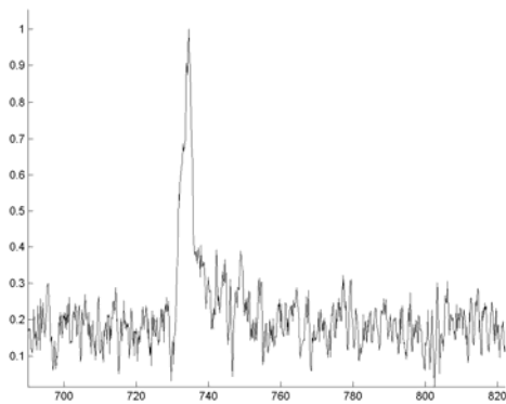
Figure 11 Reflected signal delay map over mix of bluff, hills, and farmland in North America. Horizontal axis is C/A code phase, vertical axis is correlation magnitude after 100 non-coherent summations.
