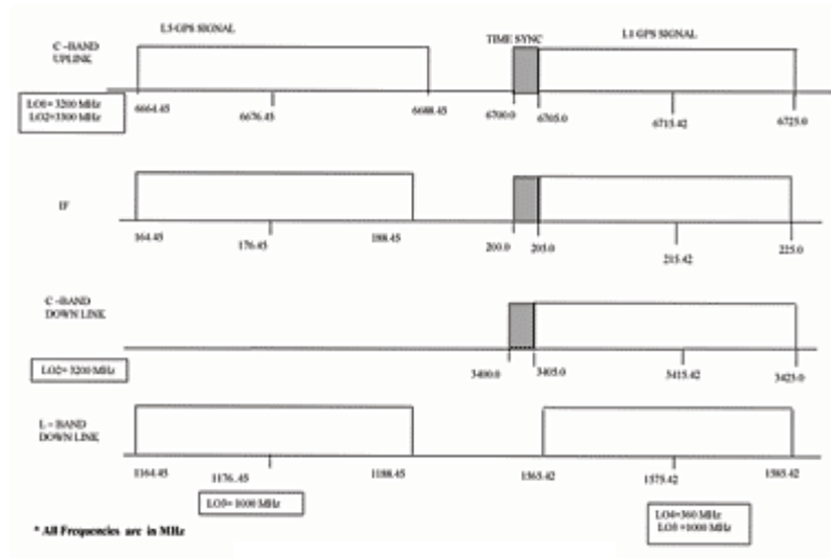
Fig. 5: Frequency Plan for the SATNAV (click for larger image)
