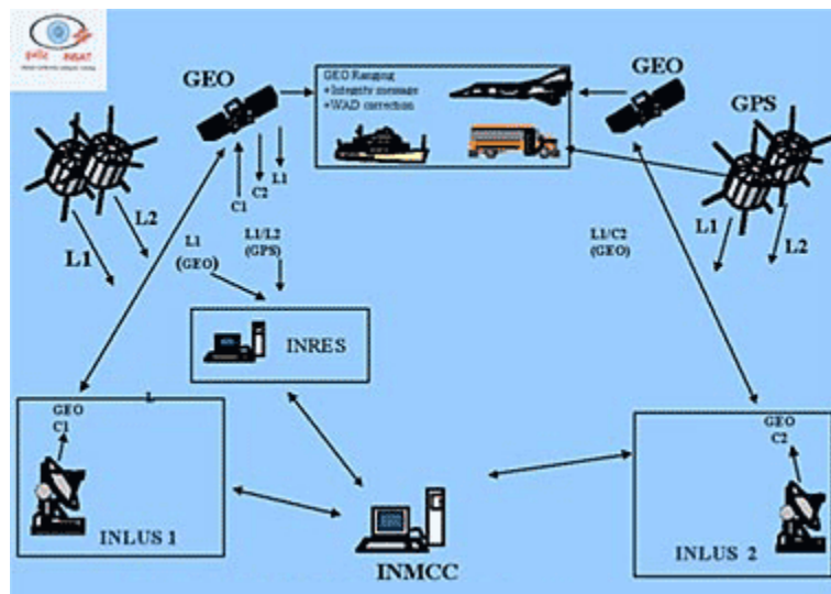
Fig. 1: WADGPS Ground Segment Concept
