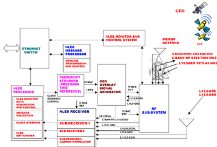
Fig. 3: Configuration of Indian Navigation Land Uplink Station
