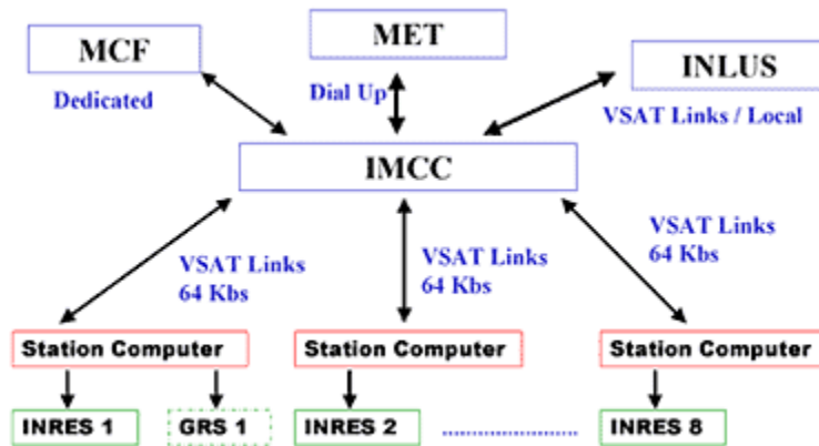
Fig. 2: Communication Interfaces
