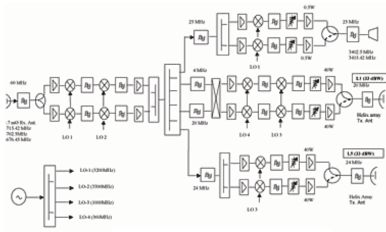
Fig. 4: Navigation Payload Schematic (click for larger image)
