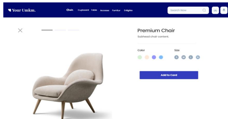
Figure 5. Web Product
