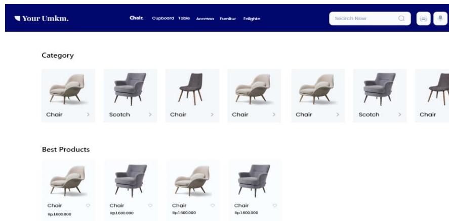
Figure 4. Web Home
