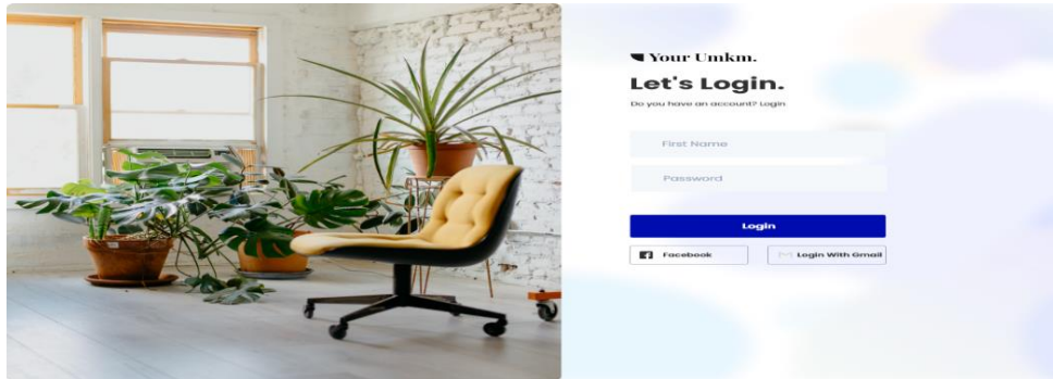
Figure 3. Web Log-in
