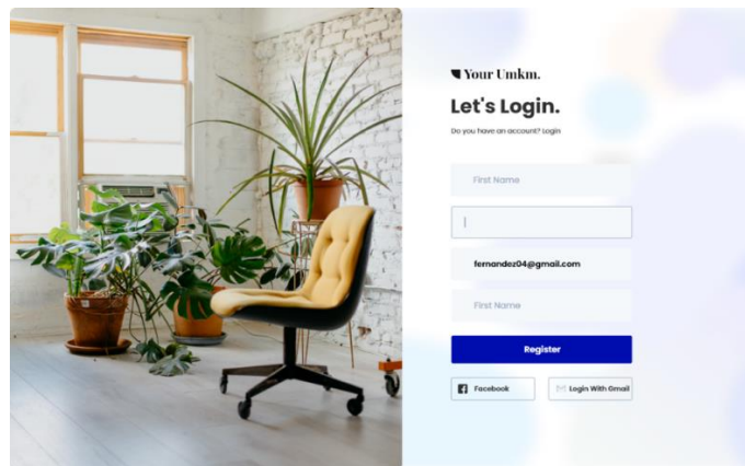
Figure 2. Web Register
