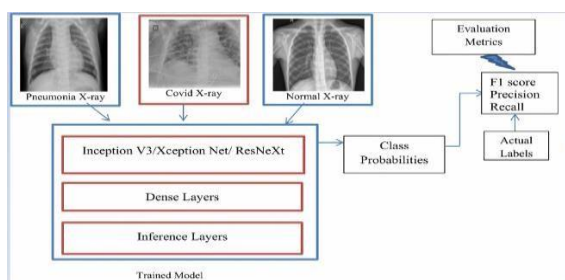
Fig. 2. The architecture of CNN model
