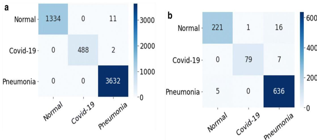
Fig. 3. Training and Testing data of the Xception model shows the confusion matrix.
