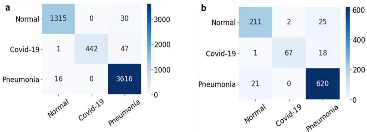
Fig. 5. Training & Testing data of the ResNeXt Model shows the confusion matrix.
