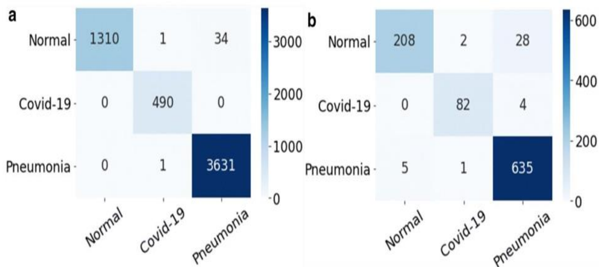
Fig. 4. Training and Testing data of Inception V3 model shows the confusion matrix.
