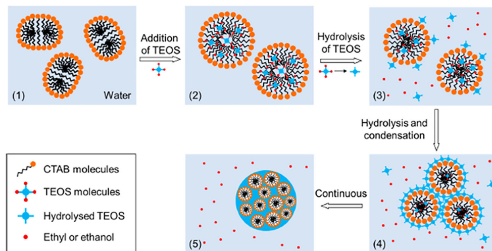
Fig. 2 Schematic of the structural changes of CTAB micelles before and after TEOS addition. (1) Before the addition of TEOS; (2) After the addition of TEOS; (3) The silica monomers are progressively released into the aqueous solution; (4) Silica monomers gradually release from the core of micelles and form a silica shell around micelles; (5) Silica forms a strong framework, and particles and mesopores are formed. (Reprinted with permission from reference 20)
