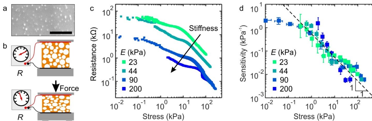
Figure 5: Conductive composite foams. (a) Optical image of the top surface of a representative conductive composite foam. Scale bar: 500 nm. (b) Schematic illustrations of composite foam compression between two electrodes, in which electric resistance is measured as a function of applied load. (c) Log-log plot of the electric resistance as a function of applied stress for conductive composite foams of different elastic moduli. (d) Log-log plot of sensitivity as a function of the applied stress, which reveals that these conductive composite foams may be used as pressure sensors that exhibit universal behavior independent of their stiffness.
