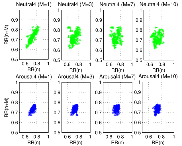
Fig. 5. Lagged Poincaré Plots from a representative subject during the elicitation of neutral (top panels) and highest arousing (bottom panels) acoustic stimuli as a function of the M lags.
