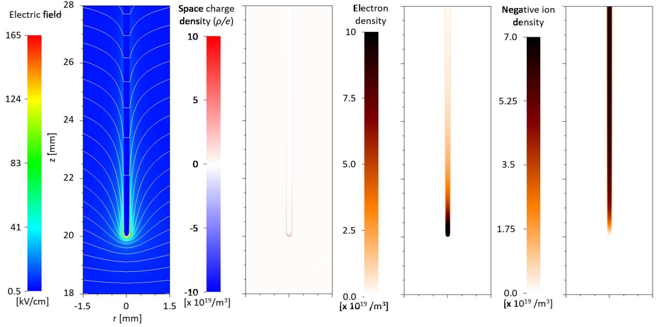
Figure 4: Plots of the 4.65 kV/cm streamer zoomed into the streamer head when it is at z = 20 mm. From left to right: (1) electric field with white equipotential lines, (2) space charge density, (3) electron density, and (4) negative ion density.
