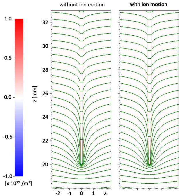
Figure 7: Charge density of the 4.65 kV/cm streamer without ion motion (left) and with ion motion (right), including green equipotential lines.
