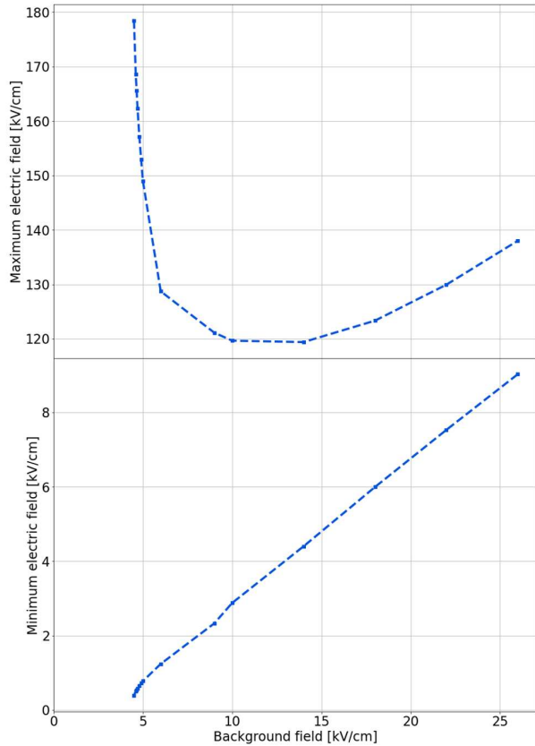
Figure 6: Maximal (top) and minimal (bottom) electric field in the streamer as a function of the background electric field. The maximal field is measured at the streamer head while the minimal field is from behind the streamer ionization front. The values were acquired when the streamer heads were at position z = 20 mm.
