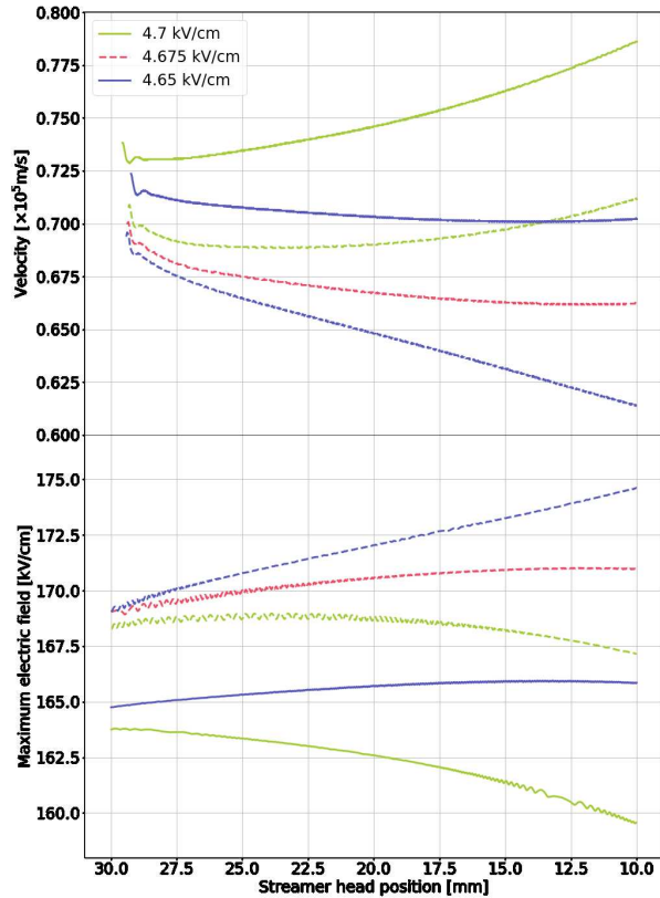
Figure 8: Velocity (top panel) and maximum electric field (bottom panel) of streamers against streamer head position for simulations with and without ion motion. Broken lines stand for simulations with ion motion. The legend on the top panel applies to the bottom panel as well.
