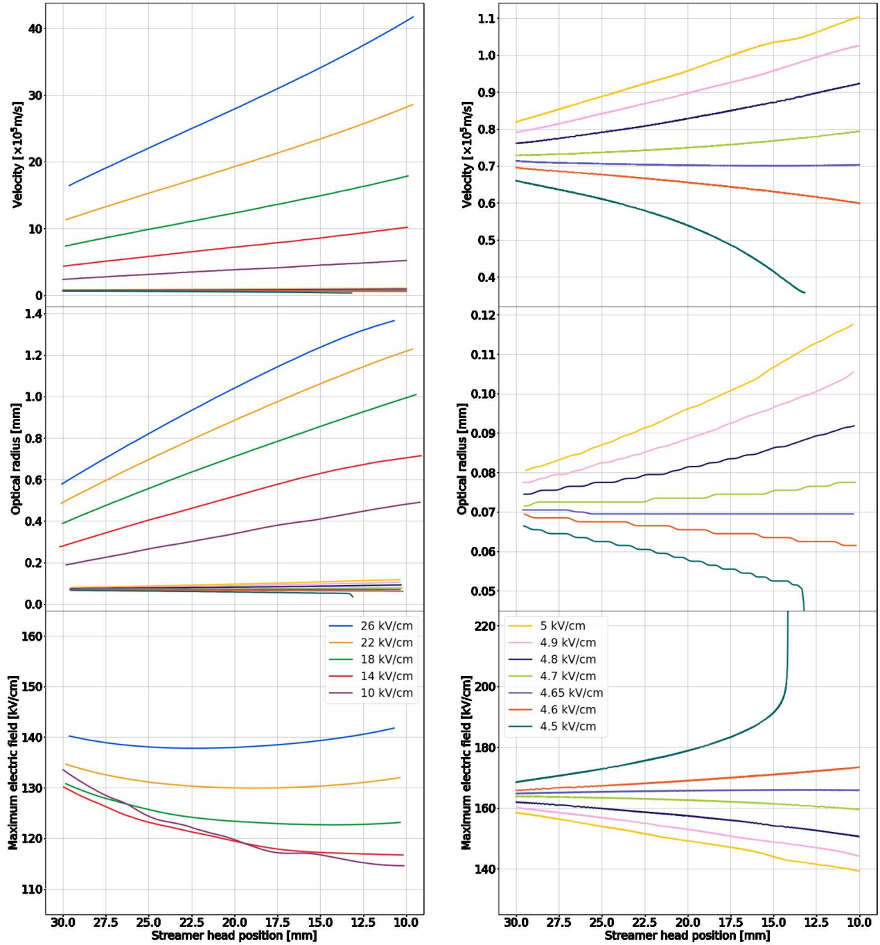
Figure 5: Properties of positive streamers as a function of length in different background fields. Top panels show the streamer velocity, middle panels the optical radius, and bottom panels the maximum electric field. Plots on the right are on a different y-axis scale and focus on the streamers in fields of 5 kV/cm and lower. Radius measurements have uncertainties of \pm 1.2 \mu\text{m} .
