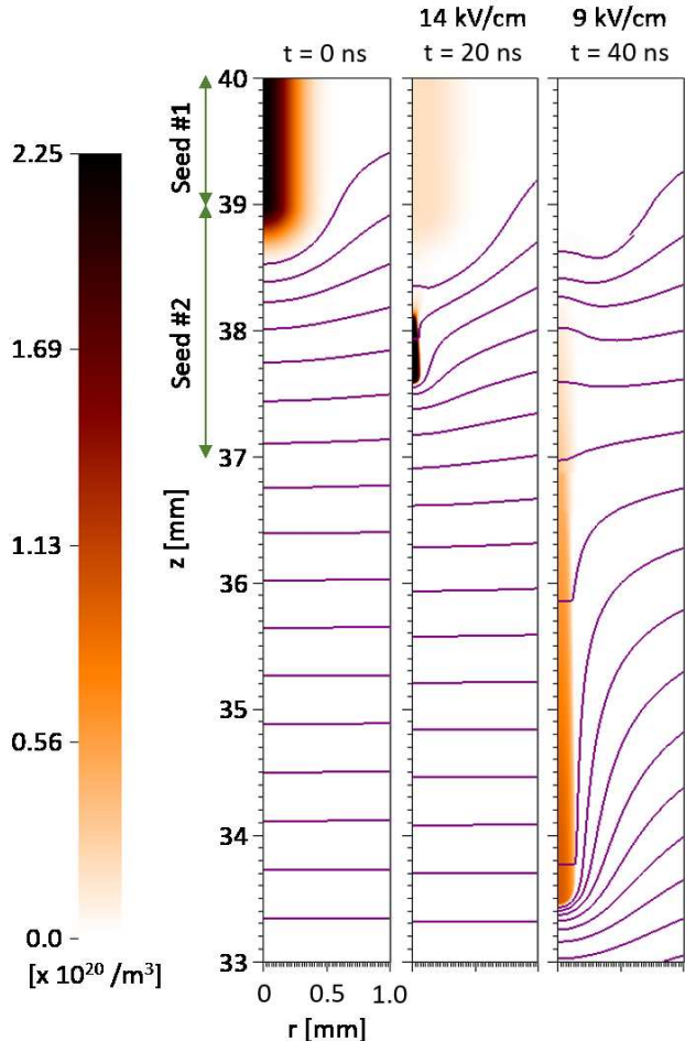
Figure 1: Initial conditions for the different background electric fields used in this paper. Shown are contour plots for the electron number densities together with purple equipotential lines. The leftmost panel is for streamers in background fields of 14 \text{ kV/cm} and higher, the middle panel is for streamers with background fields below 14 \text{ kV/cm} to 9 \text{ kV/cm} , and the rightmost panel is for streamers in fields below 9 \text{ kV/cm} . Note that the computational domain extends from 0 to 40 mm in the z direction and 0 to 20 mm in the r direction, and only a part of the domain is shown in this figure.
