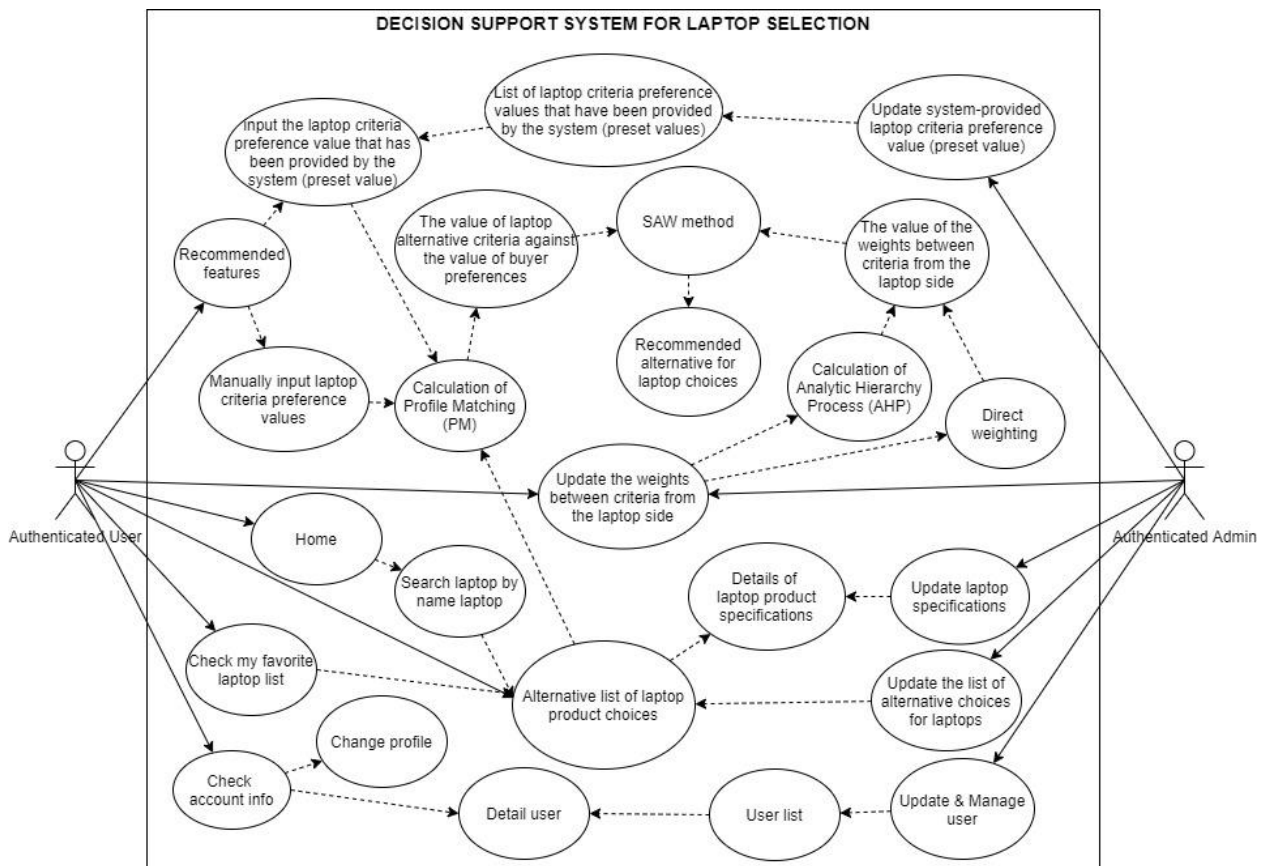
Figure 2 Use case diagram of laptop selection DSS
