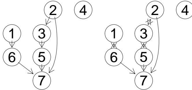
Figure 6: True DAG (left) and estimated CPDAG (right).
