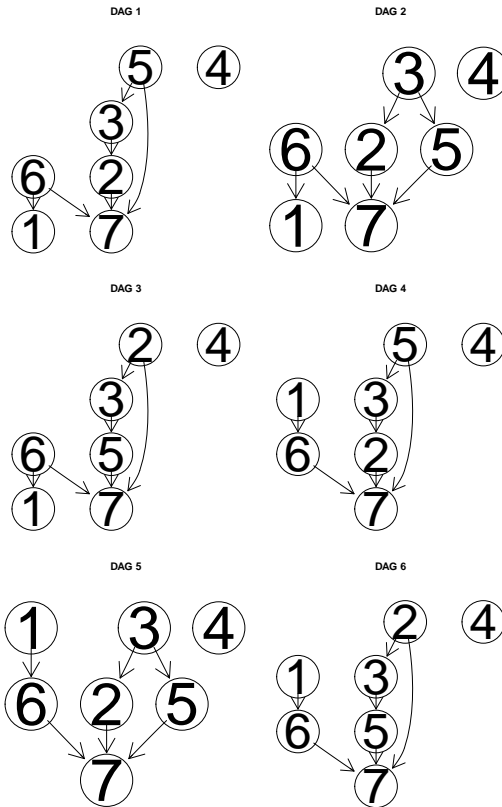
Figure 7: All DAGs belonging to the same equivalence class as the true DAG shown in Figure 6.
