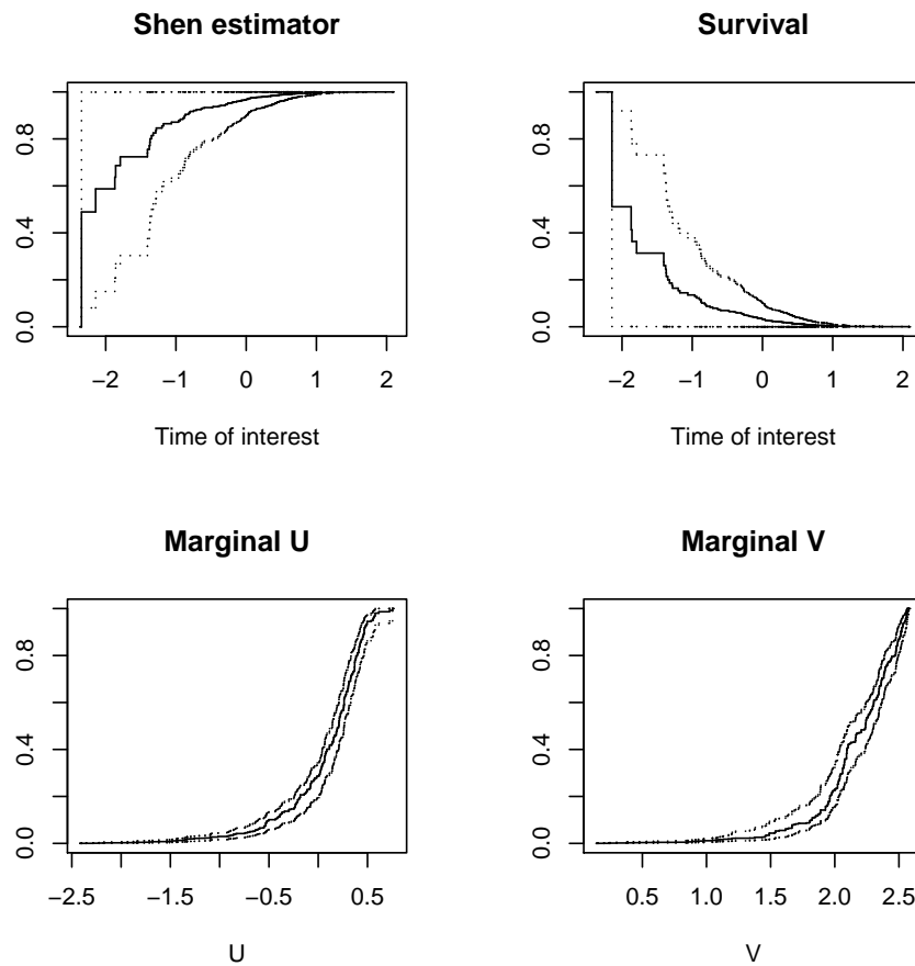
Figure 1: Cumulative DF and Survival function of quasars luminosities (top) and marginal DF of each of the truncation variables (bottom), applying shen() , with "simple" bootstrap for 95% pointwise confidence bands.
