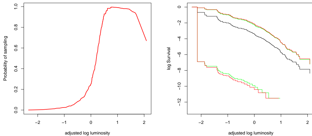
Figure 3: Bias function for the quasar data (left panel). Estimated log survival for the quasar data, using shen() function and 95% pointwise confidence bands for simple (red) and obvious (green) bootstrap methods (right panel).
