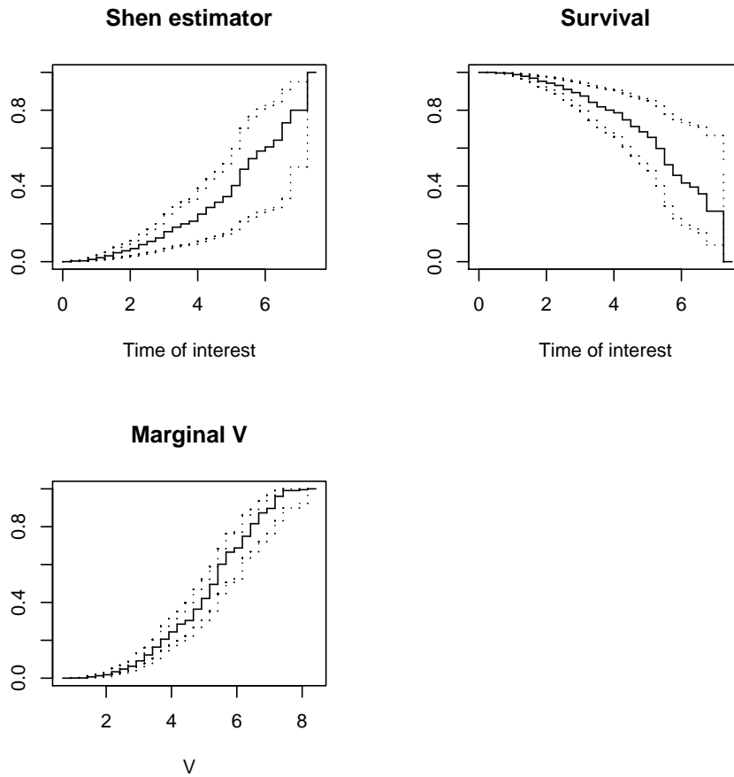
Figure 5: NPMLE obtained by shen() function for the cumulative DF and survival function of the AIDS induction times (top) and marginal DF of the right-truncation variable (bottom), together with the 95% pointwise confidence bands based on simple bootstrap method.
