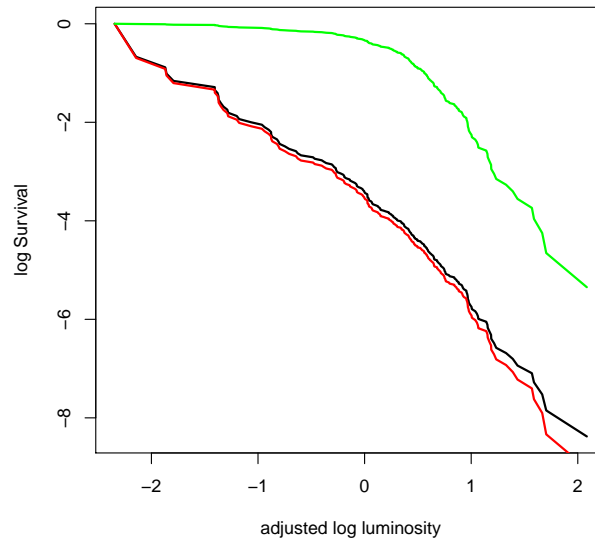
Figure 4: Estimated log survival as a function of the adjusted log luminosity evolution for the quasar data, using the NPMLE of Efron and Petrosian (black line), the Lynden-Bell estimate ignoring upper truncation (red curve), and ignoring both left and right truncation (green curve).
