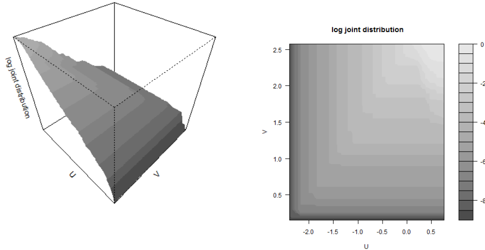
Figure 2: Bivariate distribution, in log scale of the truncation variables, for the quasar data, using option "persp" (left panel) and option option "image" (right panel).
