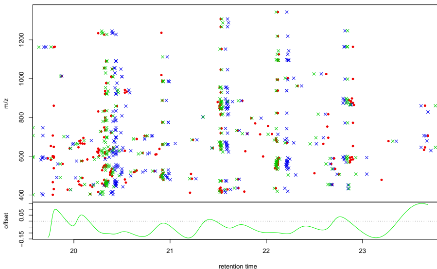
Figure 3: LC/MS alignment. Top panel: Pho4 LC/MS data at t = 5 min. Result (green) of aligning repeat 2 (blue) with repeat 3 (red). Bottom panel: estimated warping shifts.
