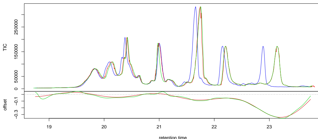
Figure 1: Top panel: TICs of the undistorted sample (blue), after distortion (red), and TIC of the sample after application of the warping estimate with amsrpm (green). Bottom panel: Time shifts for the simulated distortion (red) and the amsrpm warping estimate (green).
