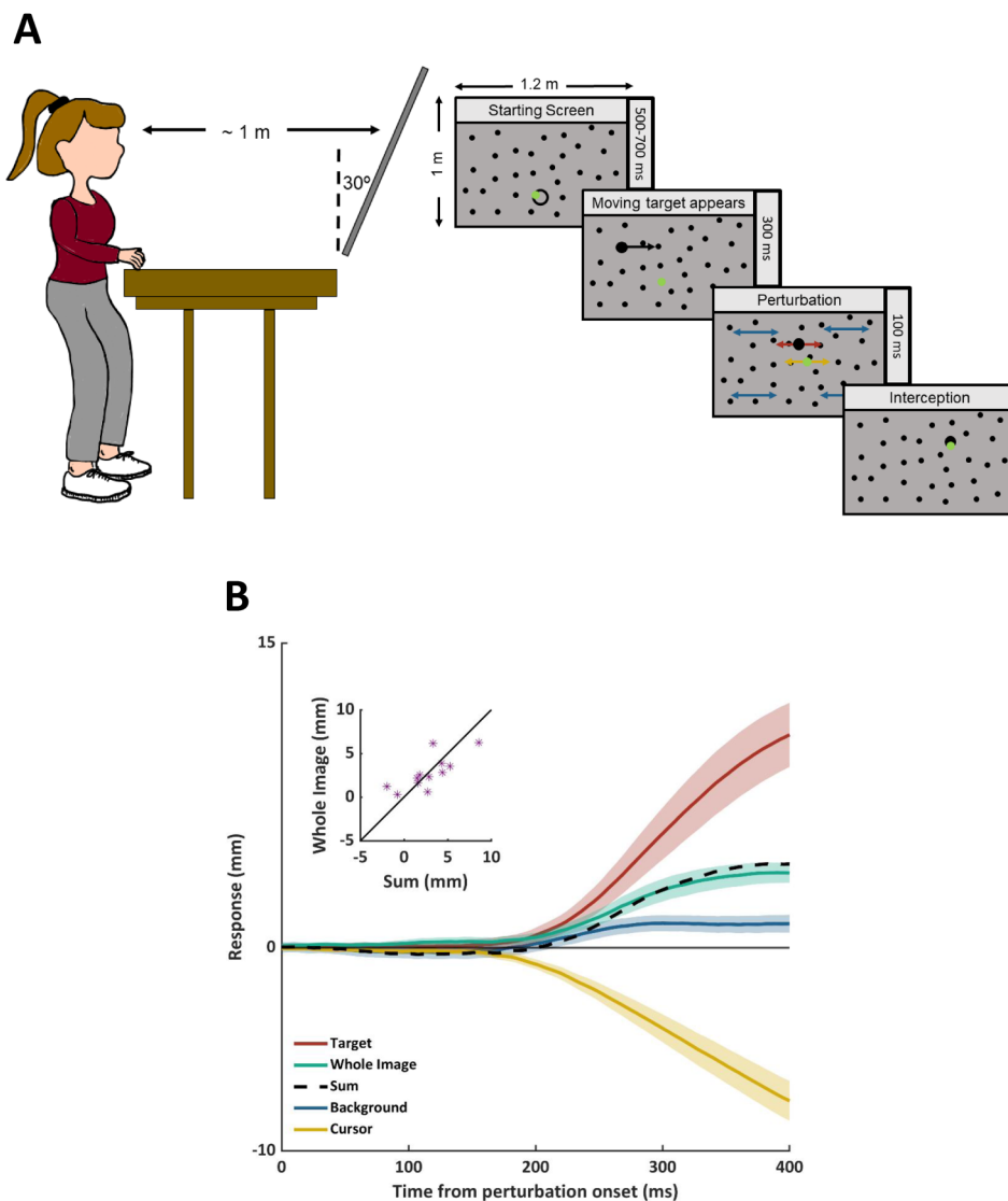
Figure 1. (a) Schematic representation of the set-up (left panel) and task (right panel). (b) Coloured curves show the average responses in each condition. A positive response is in the direction of the perturbation and a negative response is in the direction opposite the perturbation. Shaded regions show the standard error across participants. The black curve shows the sum of the average responses to the separate background, target, and cursor perturbations. The inset compares this sum with the response to the whole image moving for individual participants (300 ms after perturbation onset).
