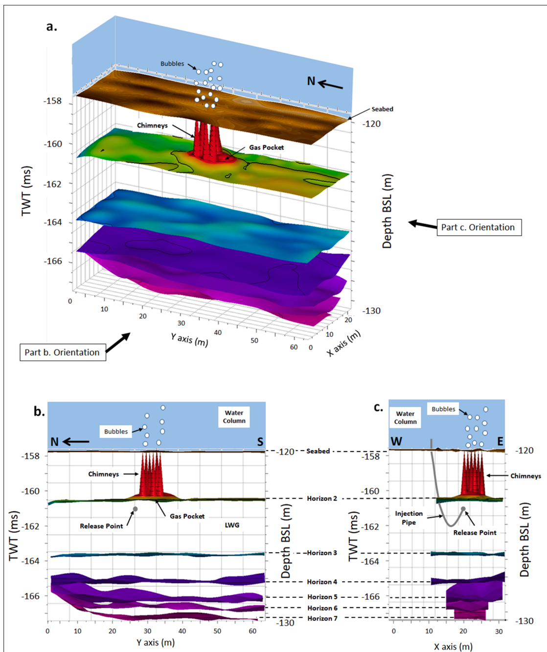
Fig. 7. 3D interpretation of seismic horizons directly beneath the release site at 143 kg/day injection rate with the resulting gas pocket and fluid escape features (chimneys) shown in red. a. Facing NE; b. facing East, release point indicated in grey, and c. facing north, release point and injection pipe indicated in grey. Data is presented in two-way travel time (TWT) with the equivalent depth below sea level (BSL) provided.
