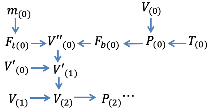
FIGURE 7. Rolled out graph for the dynamic model in figure 3 - subscripts in parentheses indicate time steps
