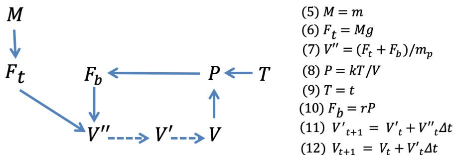
FIGURE 3. Dynamic Causal Model for Ideal Gas System
