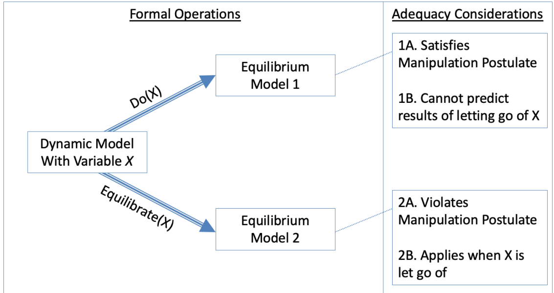
FIGURE 1. High-level map of models, operations and adequacy considerations. Adequacy considerations concern the ability of the models to predict how the system will change in response to the actions modeled by the formal operations. Considering intervening without “letting go” leads one to illegitimately privilege 1A and 2A over 1B and 2B.
