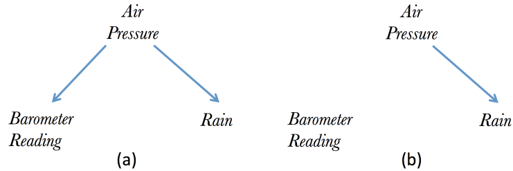
FIGURE 6. (a) Causal Graph for Barometer example (b) An Intervention on Barometer Reading
