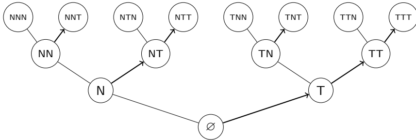
FIGURE 1. NFL for prediction. For any possible learning method (say, the method that always chooses \mathsf{T} , here represented by the arrows), there is one learning situation (path through the tree) with error 0 (follow the arrows), one with error 1 (never follow the arrow), and three situations each with error 1/3 and 2/3 . Assigning each learning situation the same probability 1/8 , the algorithm’s expected error is 1/2 .
