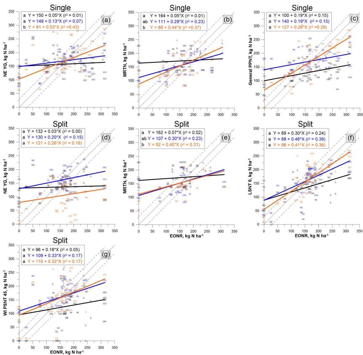
FIGURE 7 “Moderately improved” N recommendation tool improvement (i.e., good but inconsistent improvement of performance metrics across elastic net and decision tree models) for predicting the economically optimal nitrogen rate (EONR) after adjusting with soil and weather measurements. Comparison of before (black labels and lines) and after adjusting for soil and weather information using an elastic net regression (blue labels and lines) or recursive partitioning decision trees (orange labels and lines). Linear regression equations and their coefficient of variance are shown with significant differences between slopes identified with letters at the beginning of each equation. The 1:1 line is an indicator of a perfect predictor of EONR. The dashed lines represent the area in which tools were within \pm 30 \text{ kg N ha}^{-1} of EONR or relatively close to EONR. Tools were used for a “single” (at-planting) or a “split” (at-planting + sidedress) N application
