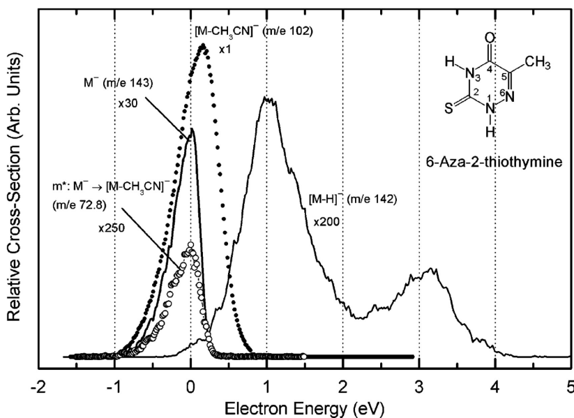
Figure 3. Anion yields as a function of electron energy for [M-\text{CH}_3\text{CN}]^- , M^- , [M-\text{H}]^- and the metastable process appearing at m/e 72.8.
