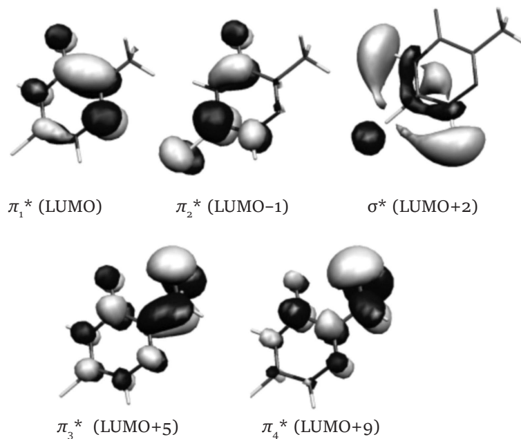
Figure 2. Molecular orbital plots of the significant virtual orbitals of 6-aza-2-thiothymine.
