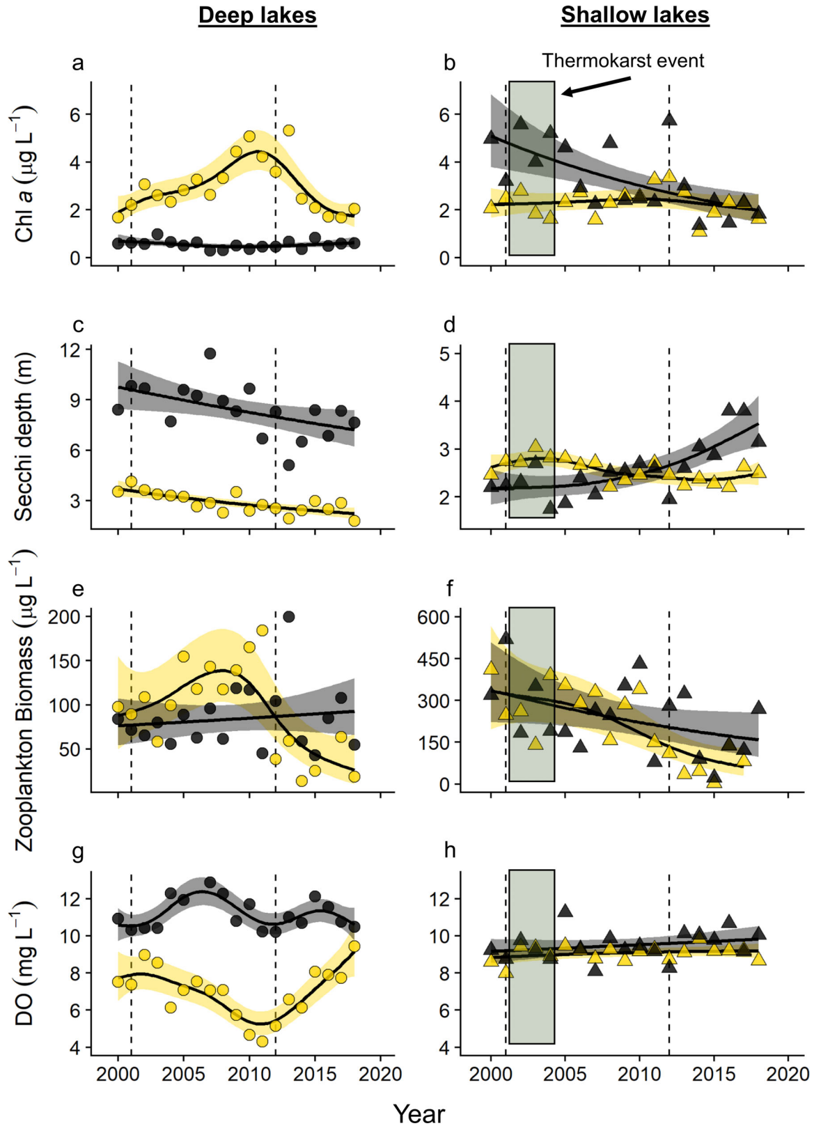
Figure 2. Epilimnetic chlorophyll a (panels a,b ), water transparency (measured as Secchi depth) (panels c,d ), zooplankton biomass (panels e,f ), and hypolimnetic dissolved oxygen measured at 8 m (panel g ) and 2 m (panel h ). Deep lakes are on the left (circles) and shallow lakes are on the right (triangles). Fertilized lakes are shown in yellow symbols, and reference lakes are in black symbols. The dashed vertical lines indicate the start and end of the fertilization treatment, and the shaded boxes in the right panels represent a natural thermokarst event we observed in the shallow, reference lake. Trend Lines are smoothing splines with 95% confidence interval shading from generalized additive models. Some y-axis scales differ among panels. Note chlorophyll a from 2000 to 2003 represents total values uncorrected for phaeophytin.
